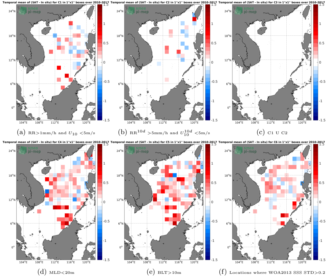
Figure 12: Temporal mean gridded over spatial boxes of size 1°x1° of \Delta SSS (SMOS-L3-BEC-OA-V1-9DAYS-0.25DEG - Argo) for 6 different subdatasets corresponding to: RR > 1\text{mm/h} and U_{10} < 5\text{m/s} (a), RR^{10d} > 5\text{mm/h} and U_{10}^{10d} < 5\text{m/s} (b), C1 U C2 (c), MLD < 20\text{m} (d), BLT > 10\text{m} (e), Locations where WOA2013 SSS STD > 0.2 (f).
