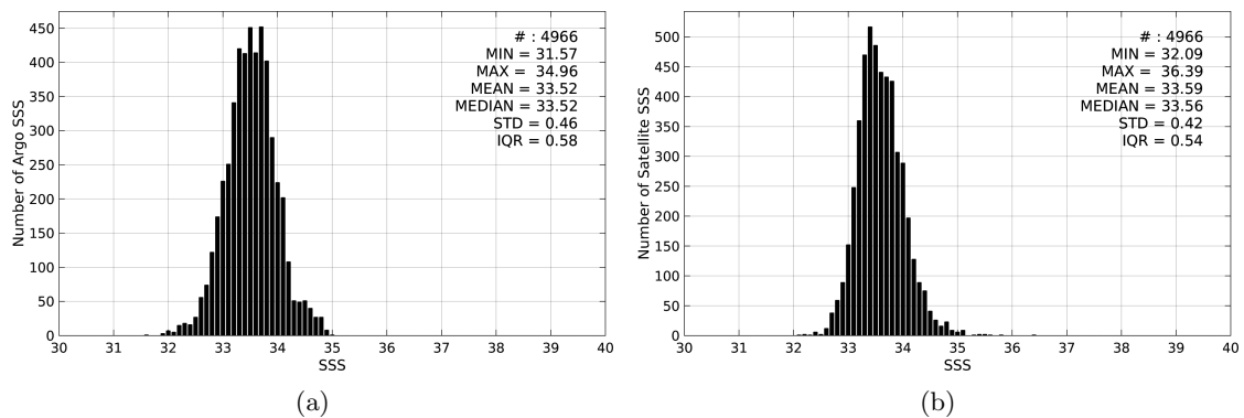
Figure 2: Histograms of SSS from Argo (a) and SMOS-L3-BEC-OA-V1-9DAYS-0.25DEG (b) considering all match-up pairs per bins of 0.1 over the South China Sea Pi-MEP region and for the full satellite product period.
