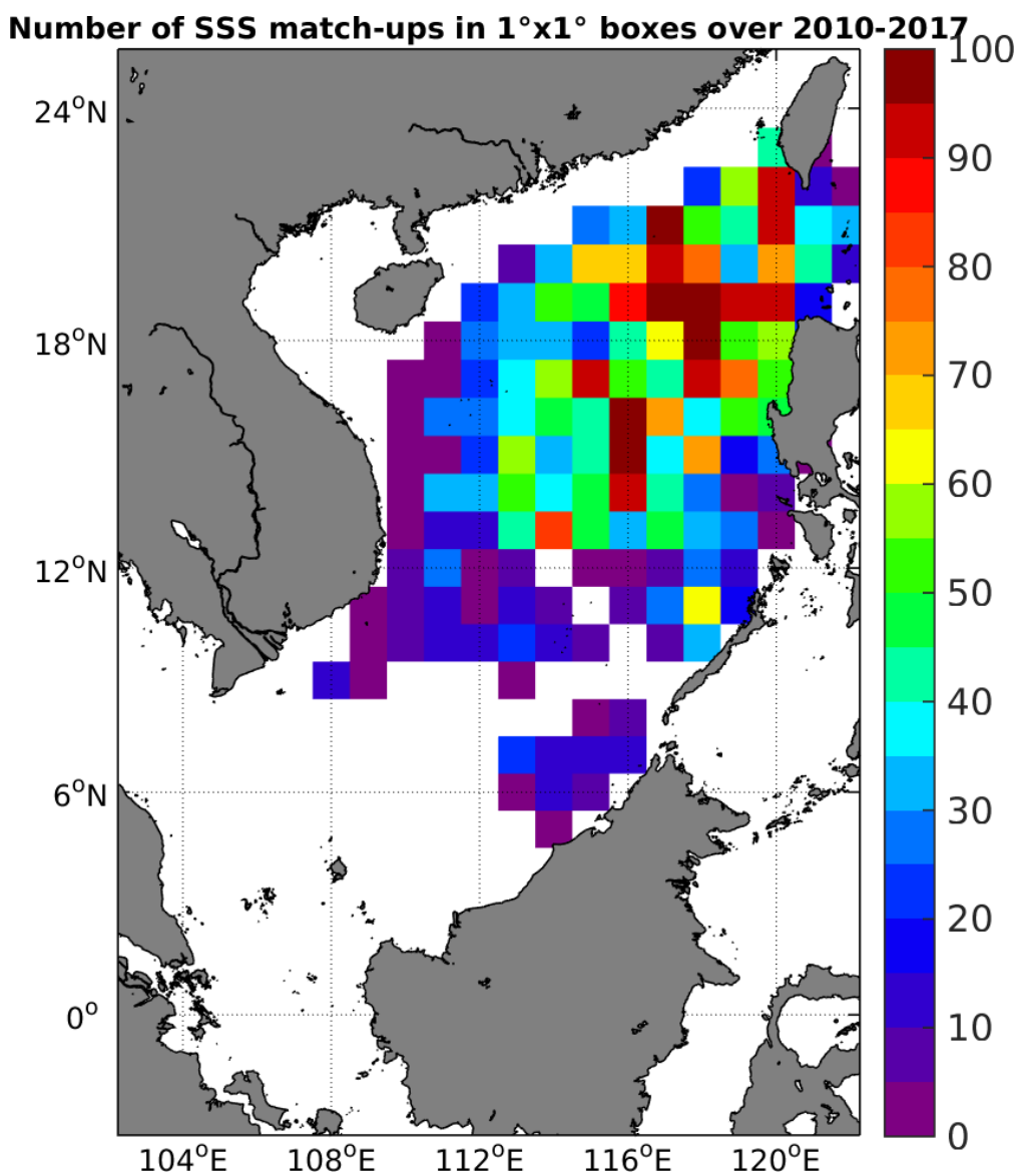
Figure 4: Number of SSS match-ups between Argo SSS and the SMOS-L3-BEC-OA-V1-9DAYS-0.25DEG SSS product for the South China Sea Pi-MEP region over 1°x1° boxes and for the full satellite product period.
