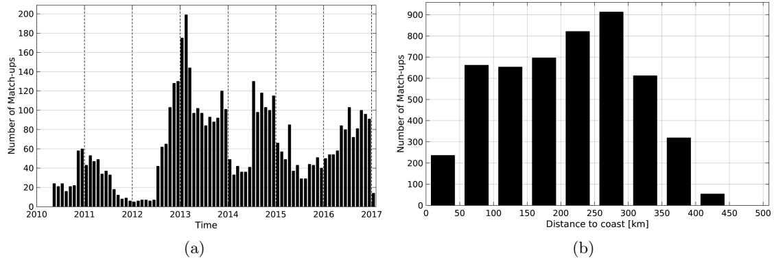
Figure 1: Number of match-ups between Argo and SMOS-L3-BEC-OA-V1-9DAYS-0.25DEG SSS as a function of time (a) and as function of the distance to coast (b) over the South China Sea Pi-MEP region and for the full satellite product period.
