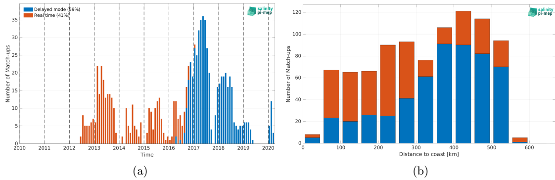
Figure 2: Number of match-ups between Argo and SMOS SSS L2-AVERAGED v700 (ESA) SSS as a function of time (a) and as function of the distance to coast (b) over the South China Sea Pi-MEP region and for the full satellite product period.
