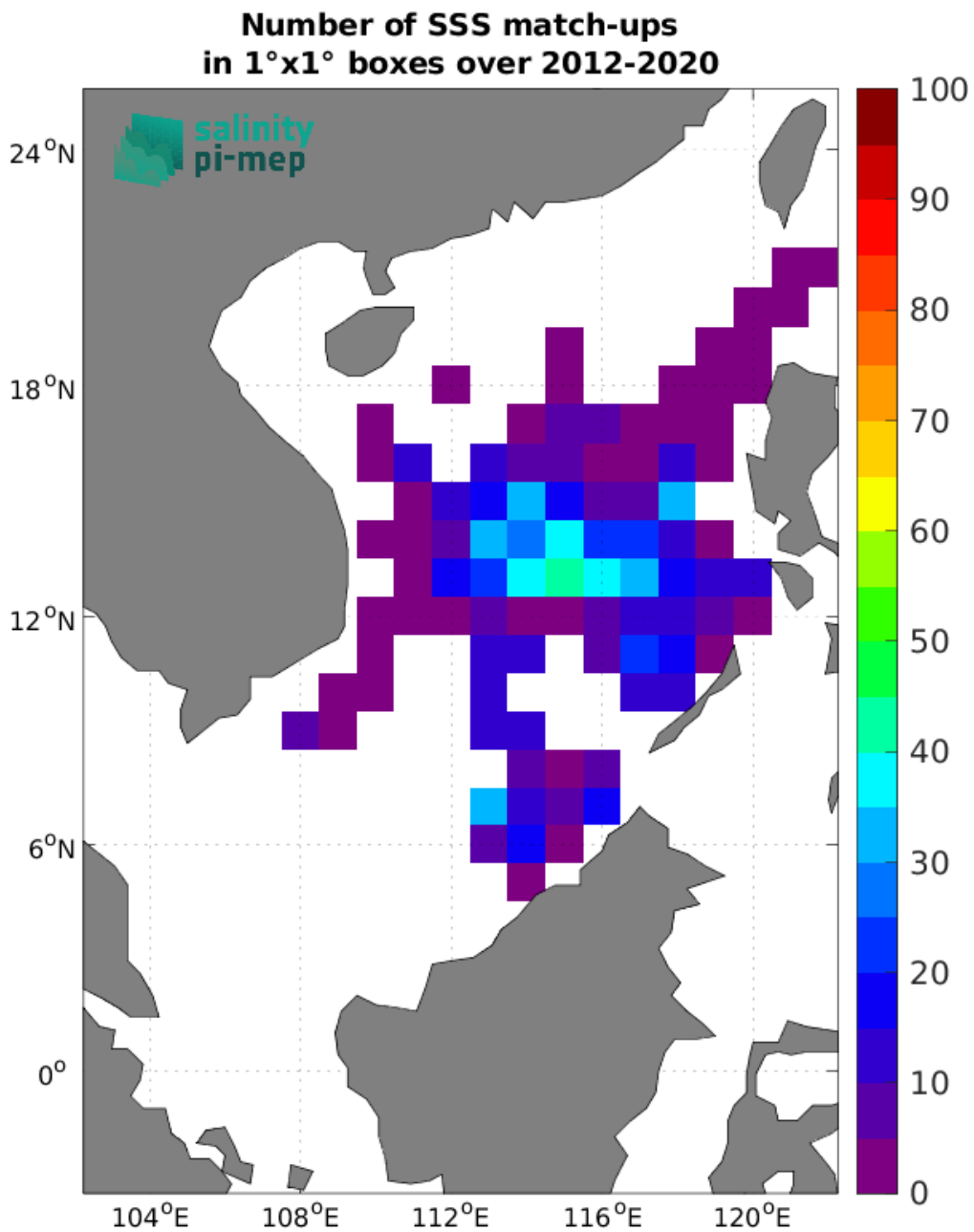
Figure 5: Number of SSS match-ups between Argo SSS and the SMOS SSS L2-AVERAGED v700 (ESA) SSS product for the South China Sea Pi-MEP region over 1^{\circ} \times 1^{\circ} boxes and for the full satellite product period.
