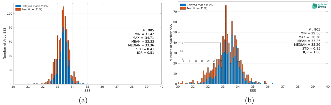
Figure 3: Histograms of SSS from Argo (a) and SMOS SSS L2-AVERAGED v700 (ESA) (b) considering all match-up pairs per bins of 0.1 over the South China Sea Pi-MEP region and for the full satellite product period.
