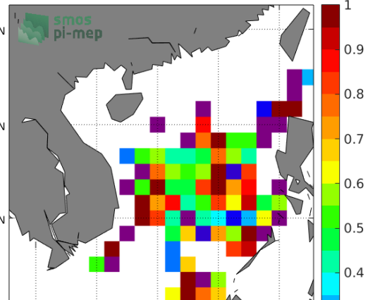
Temporal STD of (Sat - Argo) in 1°x1° boxes over 2012-2020
