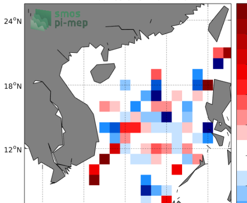
Temporal mean of (Sat - Argo) in 1°x1° boxes over 2012-2020
