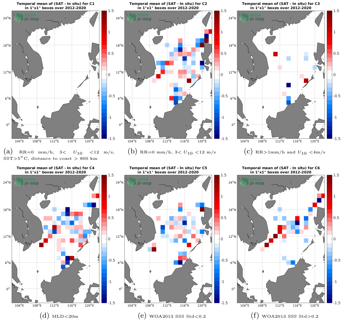
Figure 12: Temporal mean gridded over spatial boxes of size 1^\circ \times 1^\circ of \Delta SSS (SMOS SSS L2-AVERAGED v700 (ESA) - Argo) for 6 different subdatasets corresponding to: RR=0 mm/h, 3 < U_{10} < 12 m/s, SST > 5°C, distance to coast > 800 km (a), RR=0 mm/h, 3 < U_{10} < 12 m/s (b), RR > 1mm/h and U_{10} < 4 m/s (c), MLD < 20m (d), WOA2013 SSS Std < 0.2 (e), WOA2013 SSS Std > 0.2 (f).
