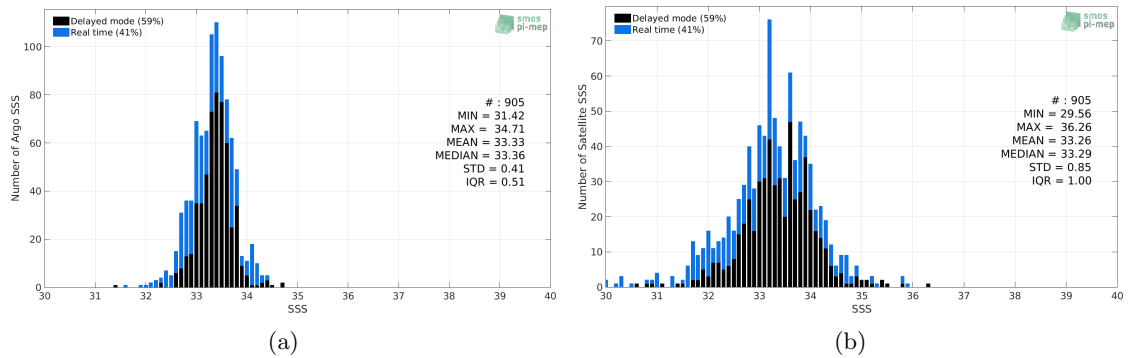
Figure 2: Histograms of SSS from Argo (a) and SMOS SSS L2-AVERAGED v700 (ESA) (b) considering all match-up pairs per bins of 0.1 over the South China Sea Pi-MEP region and for the full satellite product period.
