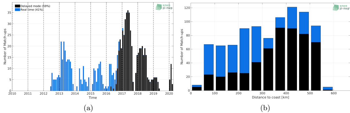
Figure 1: Number of match-ups between Argo and SMOS SSS L2-AVERAGED v700 (ESA) SSS as a function of time (a) and as function of the distance to coast (b) over the South China Sea Pi-MEP region and for the full satellite product period.
