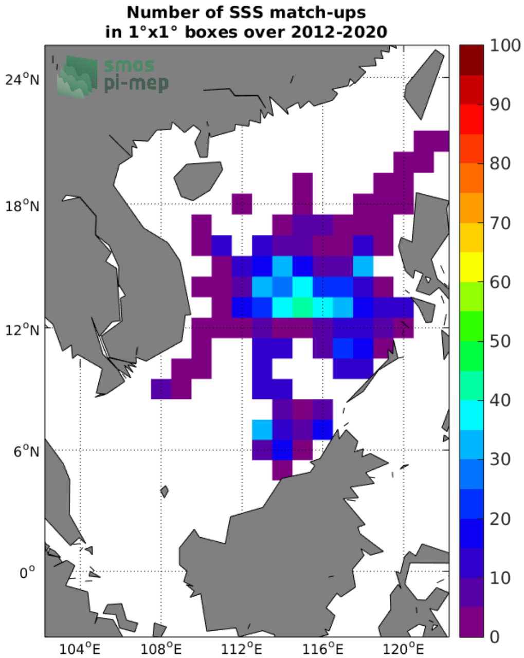
Figure 4: Number of SSS match-ups between Argo SSS and the SMOS SSS L2-AVERAGED v700 (ESA) SSS product for the South China Sea Pi-MEP region over 1°×1° boxes and for the full satellite product period.
