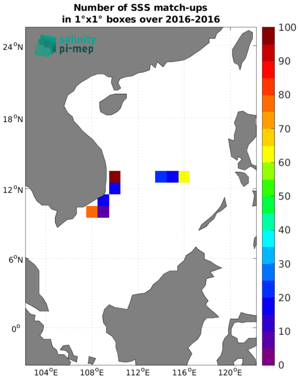
Figure 5: Number of SSS match-ups between TSG (SAMOS) SSS and the SMOS SSS L2 v700 (ESA) SSS product for the South China Sea Pi-MEP region over 1°x1° boxes and for the full satellite product period.
