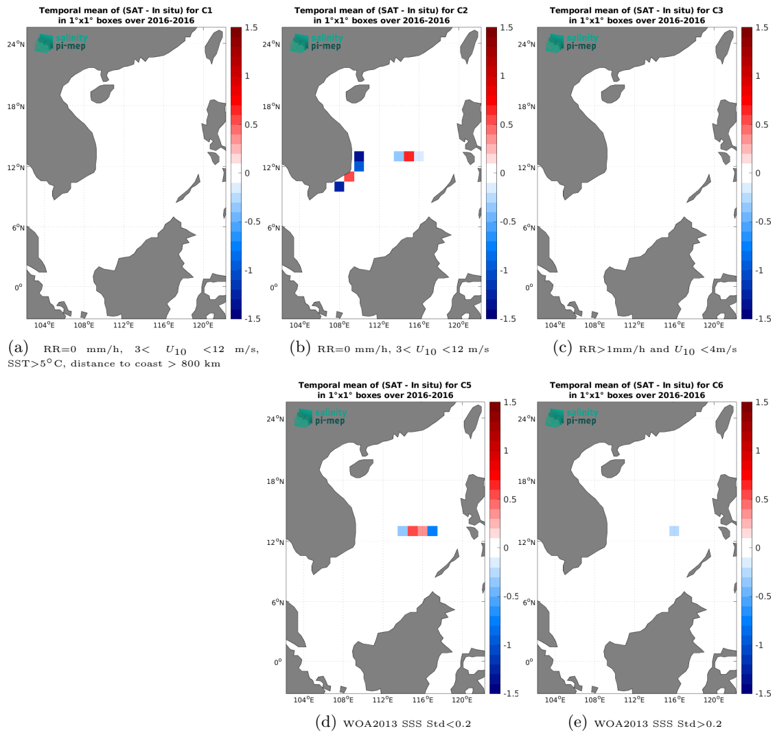
Figure 14: Temporal mean gridded over spatial boxes of size 1^\circ \times 1^\circ of \Delta SSS (SMOS SSS L2 v700 (ESA) - TSG (SAMOS)) for 5 different subdatasets corresponding to:RR=0 mm/h, 3 < U_{10} < 12 m/s, SST>5°C, distance to coast > 800 km (a), RR=0 mm/h, 3 < U_{10} < 12 m/s (b), RR>1mm/h and U_{10} < 4 m/s (c), WOA2013 SSS Std<0.2 (d), WOA2013 SSS Std>0.2 (e).
