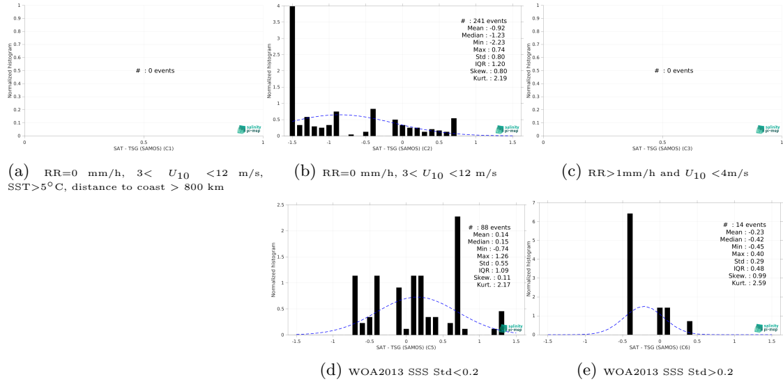
Figure 13: Normalized histogram of \Delta\text{SSS} (SMOS SSS L2 v700 (ESA) - TSG (SAMOS)) for 5 different subdatasets corresponding to: RR=0 mm/h, 3 < U_{10} < 12 m/s, SST >5^\circ\text{C} , distance to coast > 800 km (a), RR=0 mm/h, 3 < U_{10} < 12 m/s (b), RR >1 mm/h and U_{10} < 4 m/s (c), WOA2013 SSS Std <0.2 (d), WOA2013 SSS Std >0.2 (e).
