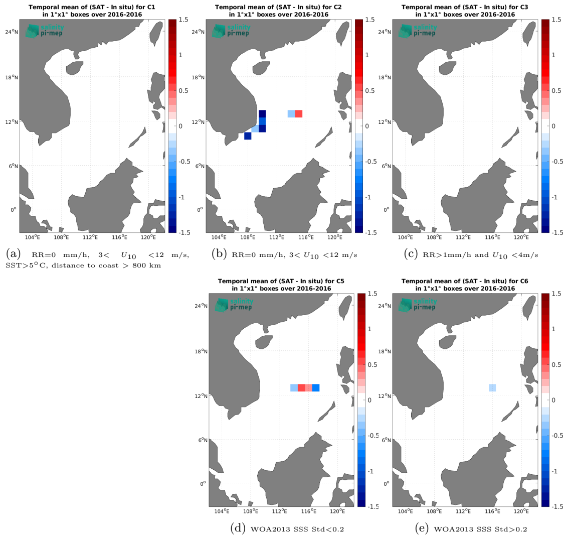
Figure 12: Temporal mean gridded over spatial boxes of size 1^\circ \times 1^\circ of \Delta\text{SSS} (SMOS SSS L2 v700 (ESA) - TSG (SAMOS)) for 5 different subdatasets corresponding to:RR=0 mm/h, 3 < U_{10} < 12 m/s, SST >5^\circ\text{C} , distance to coast > 800 km (a), RR=0 mm/h, 3 < U_{10} < 12 m/s (b), RR >1 mm/h and U_{10} < 4 m/s (c), WOA2013 SSS Std <0.2 (d), WOA2013 SSS Std >0.2 (e).
