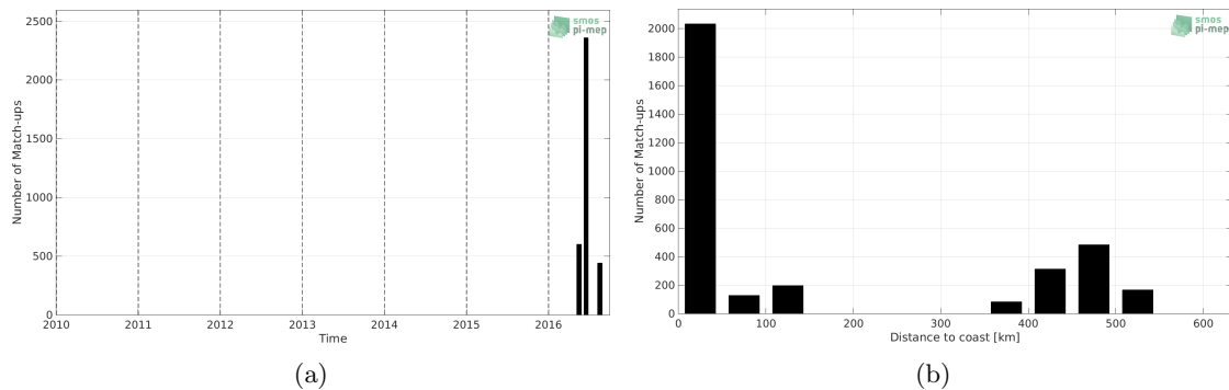
Figure 1: Number of match-ups between TSG (SAMOS) and SMOS SSS L2 v700 (ESA) SSS as a function of time (a) and as function of the distance to coast (b) over the South China Sea Pi-MEP region and for the full satellite product period.
