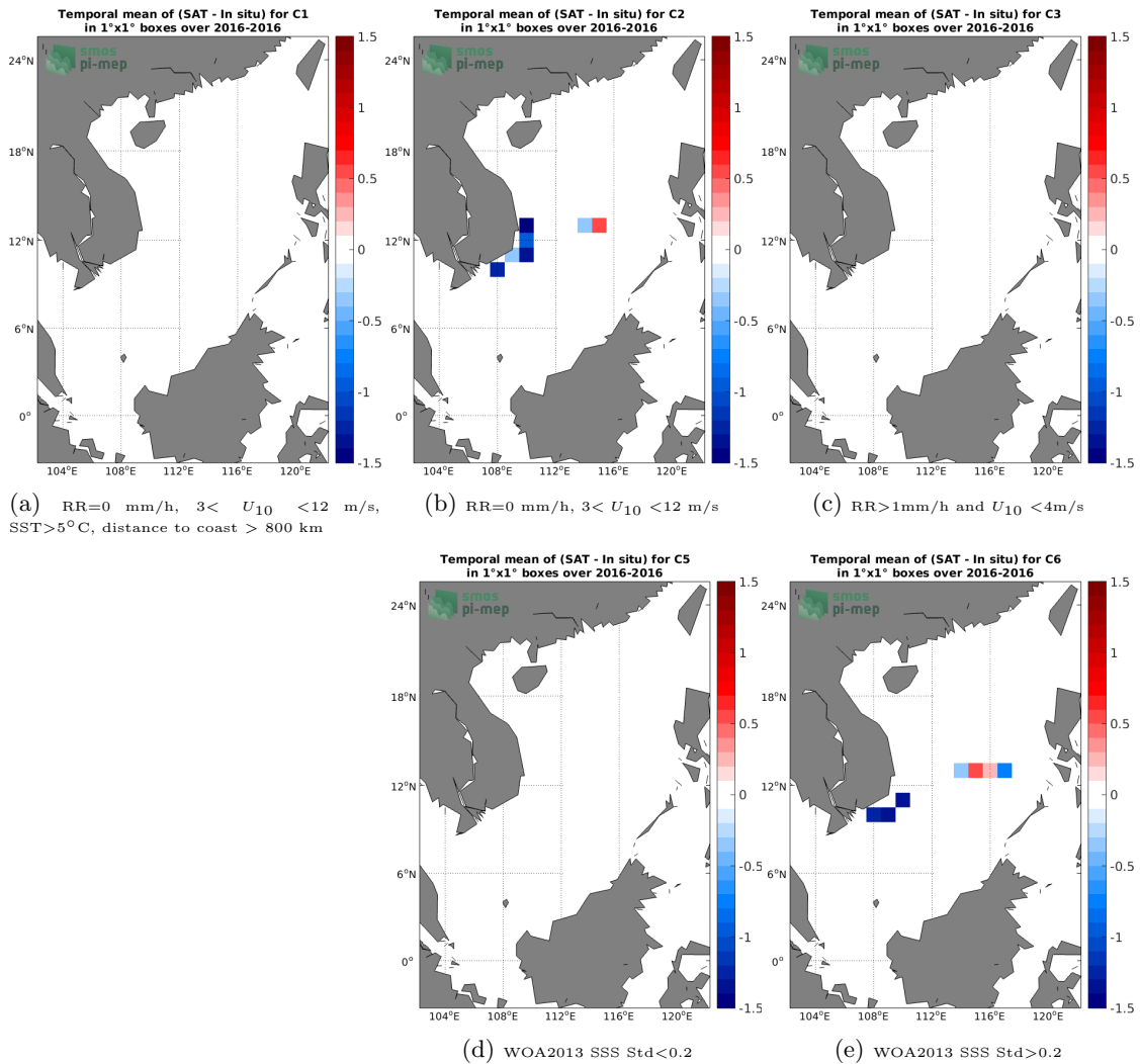
Figure 12: Temporal mean gridded over spatial boxes of size 1^\circ \times 1^\circ of \Delta SSS (SMOS SSS L2 v700 (ESA) - TSG (SAMOS)) for 5 different subdatasets corresponding to:RR=0 mm/h, 3 < U_{10} < 12 m/s, SST>5°C, distance to coast > 800 km (a), RR=0 mm/h, 3 < U_{10} < 12 m/s (b), RR>1mm/h and U_{10} < 4 m/s (c), WOA2013 SSS Std<0.2 (d), WOA2013 SSS Std>0.2 (e).
