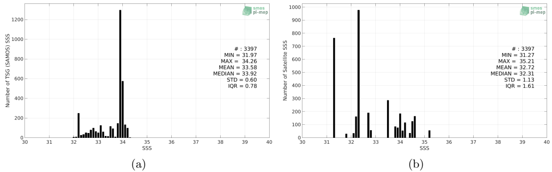
Figure 2: Histograms of SSS from TSG (SAMOS) (a) and SMOS SSS L2 v700 (ESA) (b) considering all match-up pairs per bins of 0.1 over the South China Sea Pi-MEP region and for the full satellite product period.
