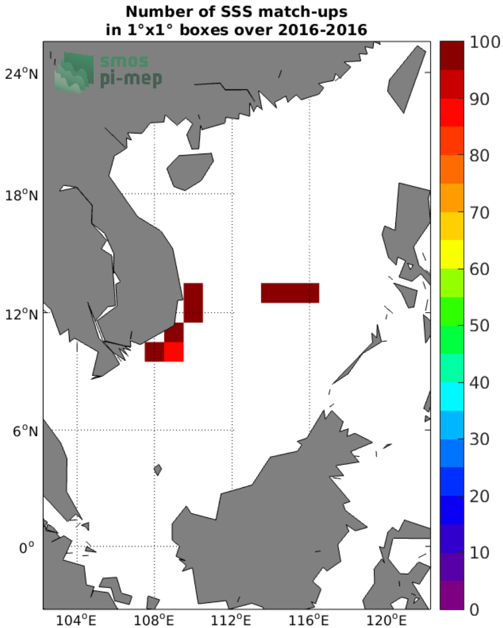
Figure 4: Number of SSS match-ups between TSG (SAMOS) SSS and the SMOS SSS L2 v700 (ESA) SSS product for the South China Sea Pi-MEP region over 1°x1° boxes and for the full satellite product period.
