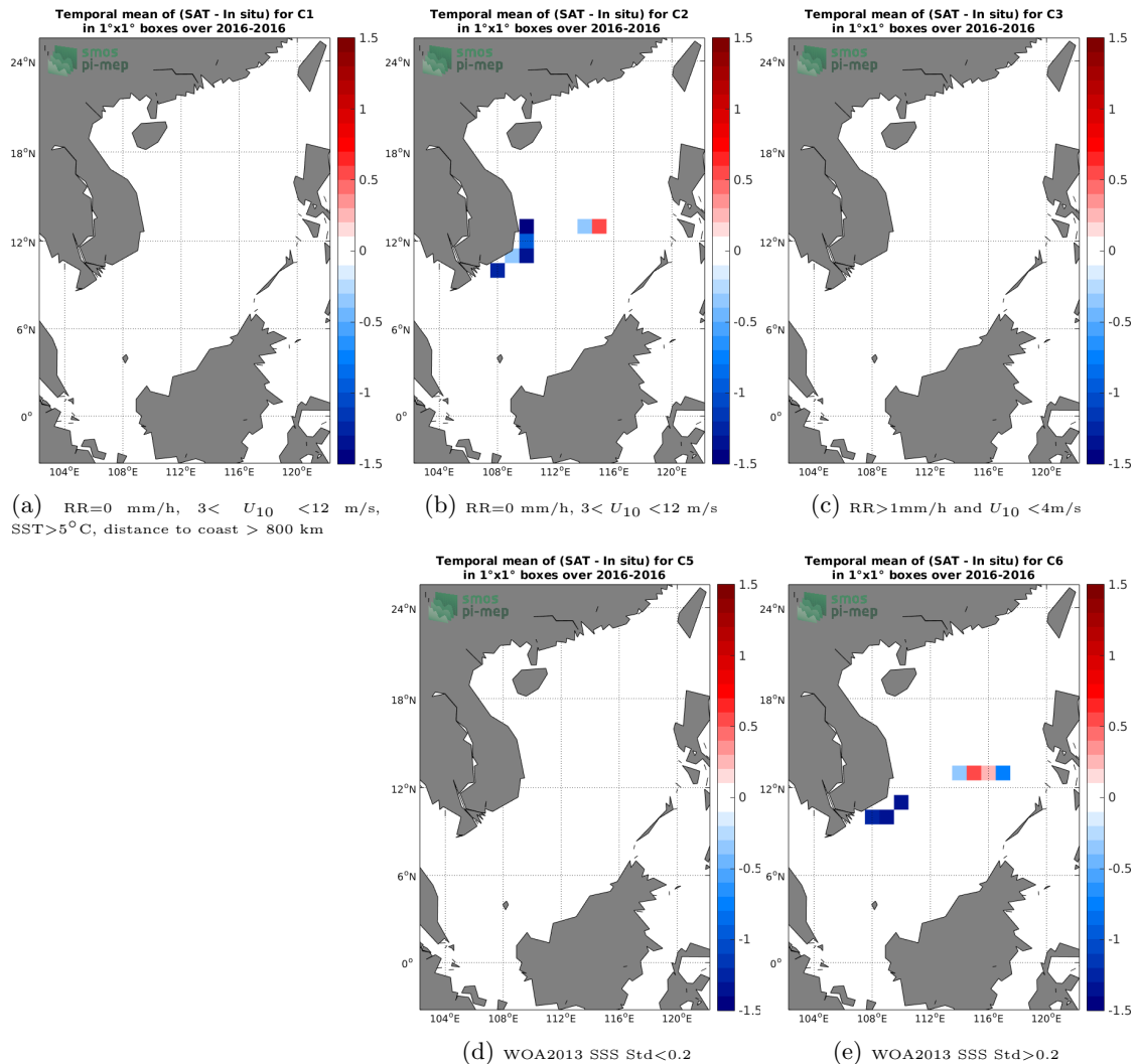
Figure 12: Temporal mean gridded over spatial boxes of size 1°x1° of \Delta SSS (SMOS SSS L2 v700 (ESA) - TSG (SAMOS)) for 5 different subdatasets corresponding to: RR=0 mm/h, 3 < U_{10} < 12 m/s, SST > 5°C, distance to coast > 800 km (a), RR=0 mm/h, 3 < U_{10} < 12 m/s (b), RR > 1mm/h and U_{10} < 4 m/s (c), WOA2013 SSS Std < 0.2 (d), WOA2013 SSS Std > 0.2 (e).
