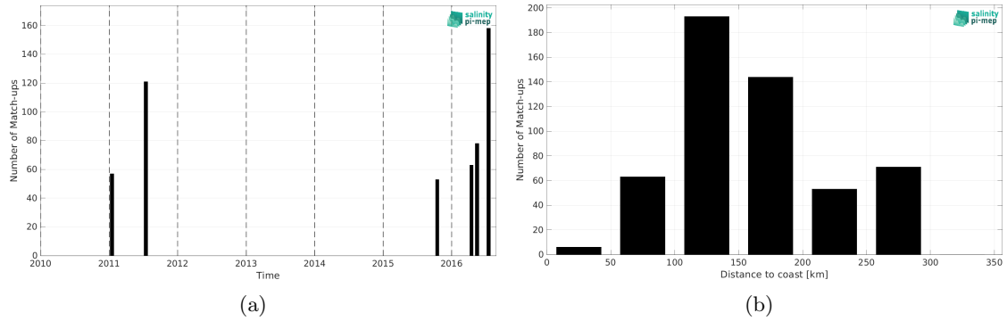
Figure 2: Number of match-ups between TSG (LEGOS-DM) and SMOS SSS L2 v700 (ESA) SSS as a function of time (a) and as function of the distance to coast (b) over the South China Sea Pi-MEP region and for the full satellite product period.
