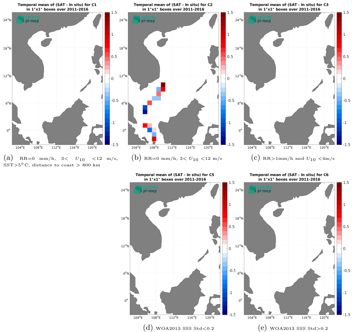
Figure 14: Temporal mean gridded over spatial boxes of size 1^\circ \times 1^\circ of \Delta\text{SSS} (SMOS SSS L2 v700 (ESA) - TSG (LEGOS-DM)) for 5 different subdatasets corresponding to: RR=0 mm/h, 3 < U_{10} < 12 m/s, SST > 5^\circ\text{C} , distance to coast > 800 km (a), RR=0 mm/h, 3 < U_{10} < 12 m/s (b), RR > 1 mm/h and U_{10} < 4 m/s (c), WOA2013 SSS Std < 0.2 (d), WOA2013 SSS Std > 0.2 (e).
