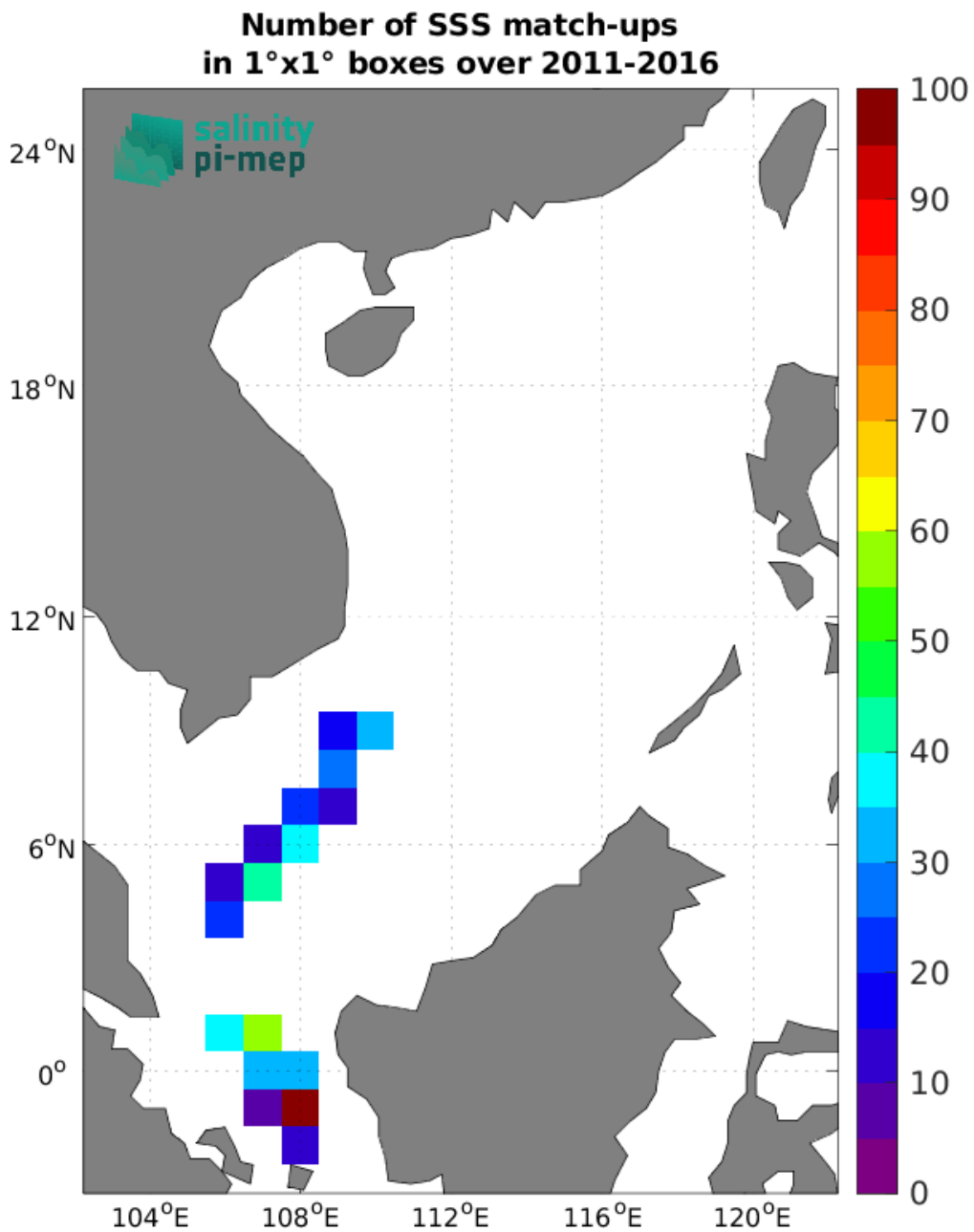
Figure 4: Number of SSS match-ups between TSG (LEGOS-DM) SSS and the SMOS SSS L2 v700 (ESA) SSS product for the South China Sea Pi-MEP region over 1^{\circ} \times 1^{\circ} boxes and for the full satellite product period.
