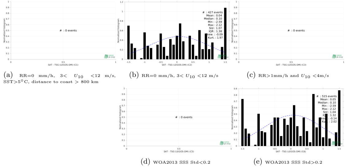
Figure 13: Normalized histogram of \Delta SSS (SMOS SSS L2 v700 (ESA) - TSG (LEGOS-DM)) for 5 different subdatasets corresponding to: RR=0 mm/h, 3 < U_{10} < 12 m/s, SST > 5°C, distance to coast > 800 km (a), RR=0 mm/h, 3 < U_{10} < 12 m/s (b), RR > 1mm/h and U_{10} < 4 m/s (c), WOA2013 SSS Std < 0.2 (d), WOA2013 SSS Std > 0.2 (e).
