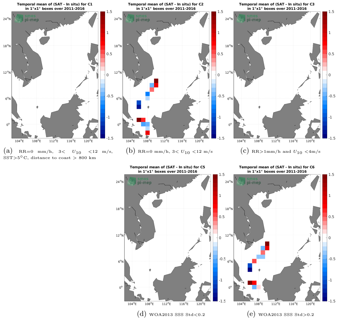
Figure 12: Temporal mean gridded over spatial boxes of size 1^\circ \times 1^\circ of \Delta SSS (SMOS SSS L2 v700 (ESA) - TSG (LEGOS-DM)) for 5 different subdatasets corresponding to:RR=0 mm/h, 3 < U_{10} < 12 m/s, SST>5°C, distance to coast > 800 km (a), RR=0 mm/h, 3 < U_{10} < 12 m/s (b), RR>1mm/h and U_{10} < 4 m/s (c), WOA2013 SSS Std<0.2 (d), WOA2013 SSS Std>0.2 (e).
