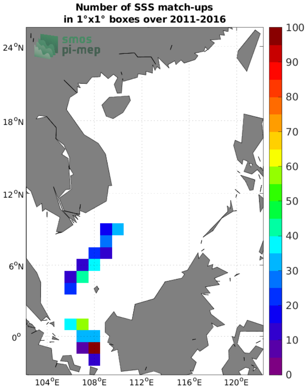
Figure 4: Number of SSS match-ups between TSG (LEGOS-DM) SSS and the SMOS SSS L2 v700 (ESA) SSS product for the South China Sea Pi-MEP region over 1°x1° boxes and for the full satellite product period.
