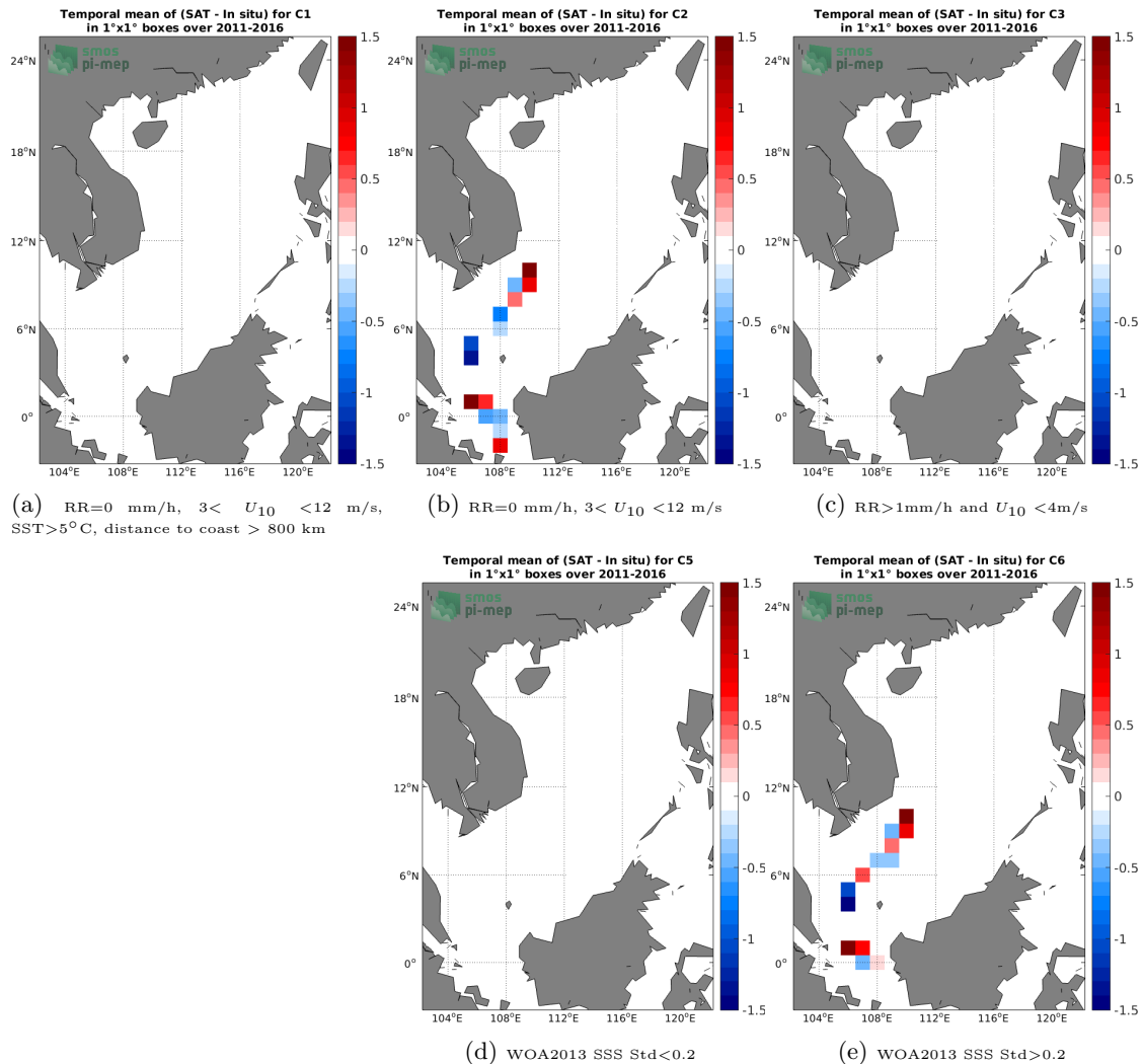
Figure 12: Temporal mean gridded over spatial boxes of size 1^\circ \times 1^\circ of \Delta\text{SSS} (SMOS SSS L2 v700 (ESA) - TSG (LEGOS-DM)) for 5 different subdatasets corresponding to: RR=0 mm/h, 3 < U_{10} < 12 m/s, SST > 5^\circ\text{C} , distance to coast > 800 km (a), RR=0 mm/h, 3 < U_{10} < 12 m/s (b), RR > 1 mm/h and U_{10} < 4 m/s (c), WOA2013 SSS Std < 0.2 (d), WOA2013 SSS Std > 0.2 (e).
