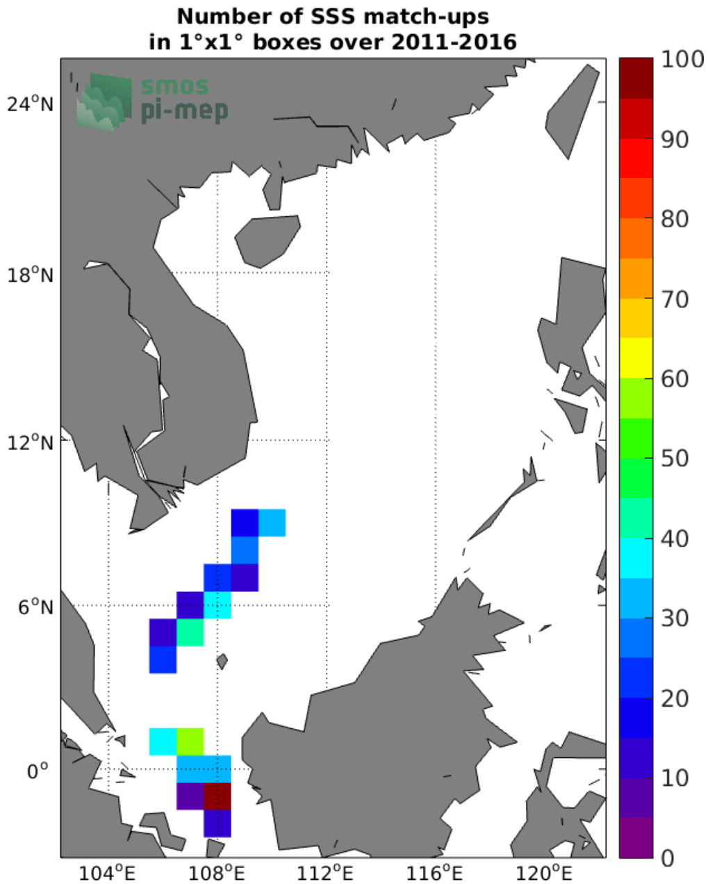
Figure 4: Number of SSS match-ups between TSG (LEGOS-DM) SSS and the SMOS SSS L2 v700 (ESA) SSS product for the South China Sea Pi-MEP region over 1^\circ \times 1^\circ boxes and for the full satellite product period.
