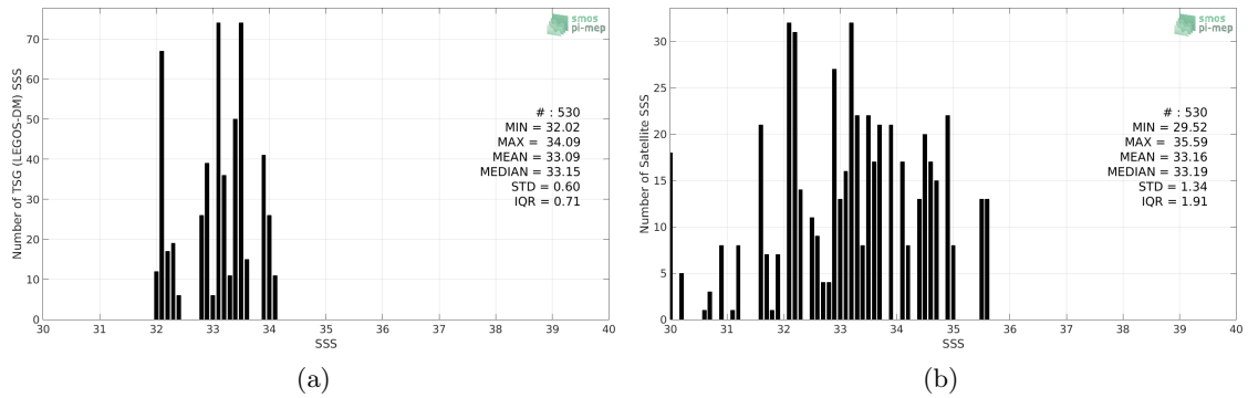
Figure 2: Histograms of SSS from TSG (LEGOS-DM) (a) and SMOS SSS L2 v700 (ESA) (b) considering all match-up pairs per bins of 0.1 over the South China Sea Pi-MEP region and for the full satellite product period.
