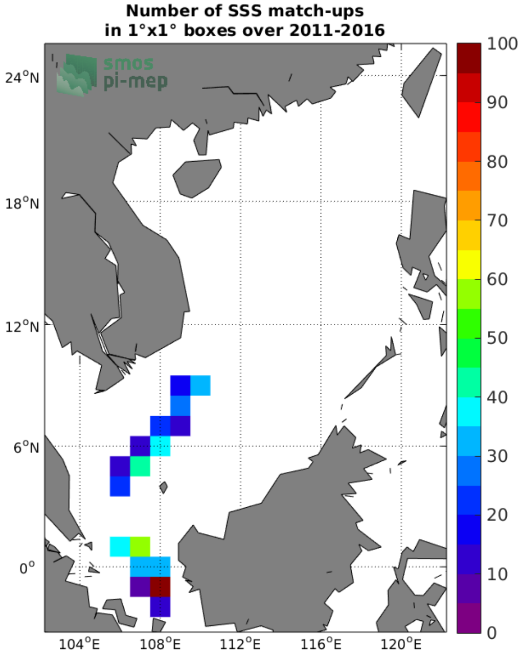
Figure 4: Number of SSS match-ups between TSG (LEGOS-DM) SSS and the SMOS SSS L2 v700 (ESA) SSS product for the South China Sea Pi-MEP region over 1°x1° boxes and for the full satellite product period.
