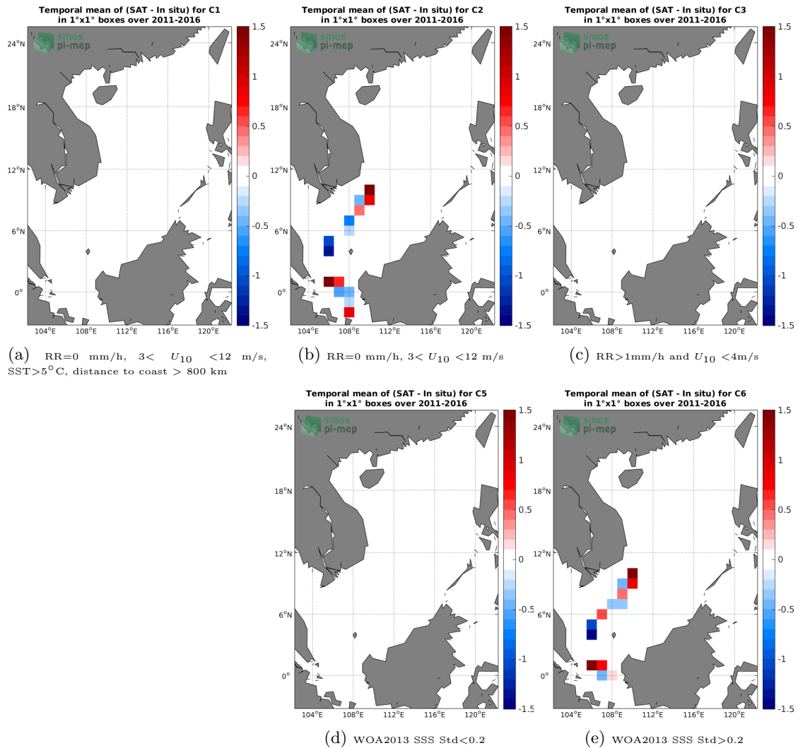
Figure 12: Temporal mean gridded over spatial boxes of size 1°x1° of \Delta SSS (SMOS SSS L2 v700 (ESA) - TSG (LEGOS-DM)) for 5 different subdatasets corresponding to: RR=0 mm/h, 3 < U_{10} < 12 m/s, SST > 5°C, distance to coast > 800 km (a), RR=0 mm/h, 3 < U_{10} < 12 m/s (b), RR > 1mm/h and U_{10} < 4 m/s (c), WOA2013 SSS Std < 0.2 (d), WOA2013 SSS Std > 0.2 (e).
