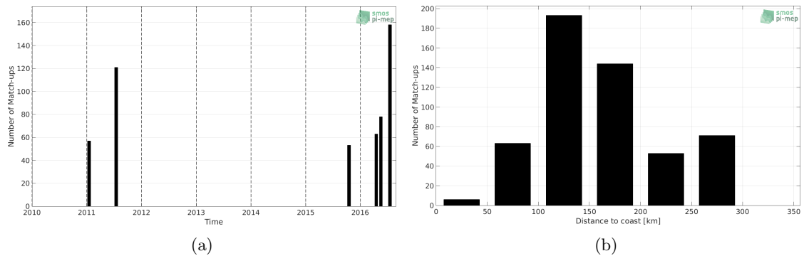
Figure 1: Number of match-ups between TSG (LEGOS-DM) and SMOS SSS L2 v700 (ESA) SSS as a function of time (a) and as function of the distance to coast (b) over the South China Sea Pi-MEP region and for the full satellite product period.
