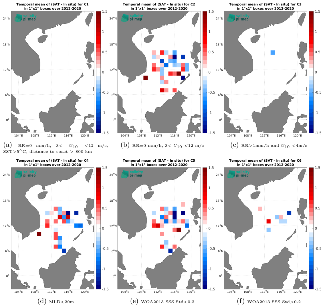
Figure 14: Temporal mean gridded over spatial boxes of size 1^\circ \times 1^\circ of \Delta SSS (SMOS SSS L2 v700 (ESA) - Argo) for 6 different subdatasets corresponding to: RR=0 mm/h, 3 < U_{10} < 12 m/s, SST>5°C, distance to coast > 800 km (a), RR=0 mm/h, 3 < U_{10} < 12 m/s (b), RR>1mm/h and U_{10} < 4 m/s (c),MLD<20m (d),WOA2013 SSS Std<0.2 (e),WOA2013 SSS Std>0.2 (f).
