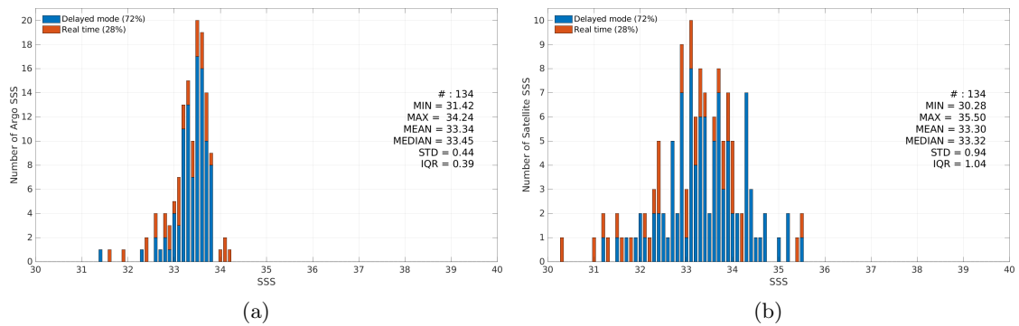
Figure 3: Histograms of SSS from Argo (a) and SMOS SSS L2 v700 (ESA) (b) considering all match-up pairs per bins of 0.1 over the South China Sea Pi-MEP region and for the full satellite product period.
