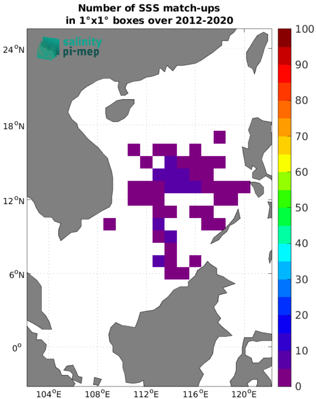
Figure 5: Number of SSS match-ups between Argo SSS and the SMOS SSS L2 v700 (ESA) SSS product for the South China Sea Pi-MEP region over 1°×1° boxes and for the full satellite product period.
