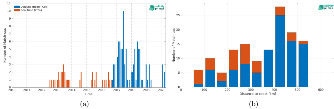
Figure 2: Number of match-ups between Argo and SMOS SSS L2 v700 (ESA) SSS as a function of time (a) and as function of the distance to coast (b) over the South China Sea Pi-MEP region and for the full satellite product period.
