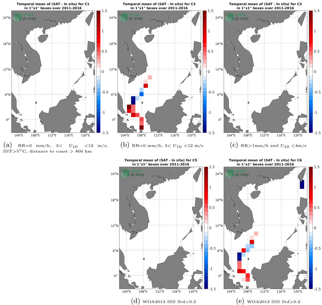
Figure 12: Temporal mean gridded over spatial boxes of size 1^\circ \times 1^\circ of \Delta SSS (SMOS SSS L2 v662 (ESA) - TSG (LEGOS-DM)) for 5 different subdatasets corresponding to:RR=0 mm/h, 3 < U_{10} < 12 m/s, SST >5^\circ C, distance to coast > 800 km (a), RR=0 mm/h, 3 < U_{10} < 12 m/s (b), RR >1 mm/h and U_{10} < 4 m/s (c), WOA2013 SSS Std <0.2 (d), WOA2013 SSS Std >0.2 (e).
