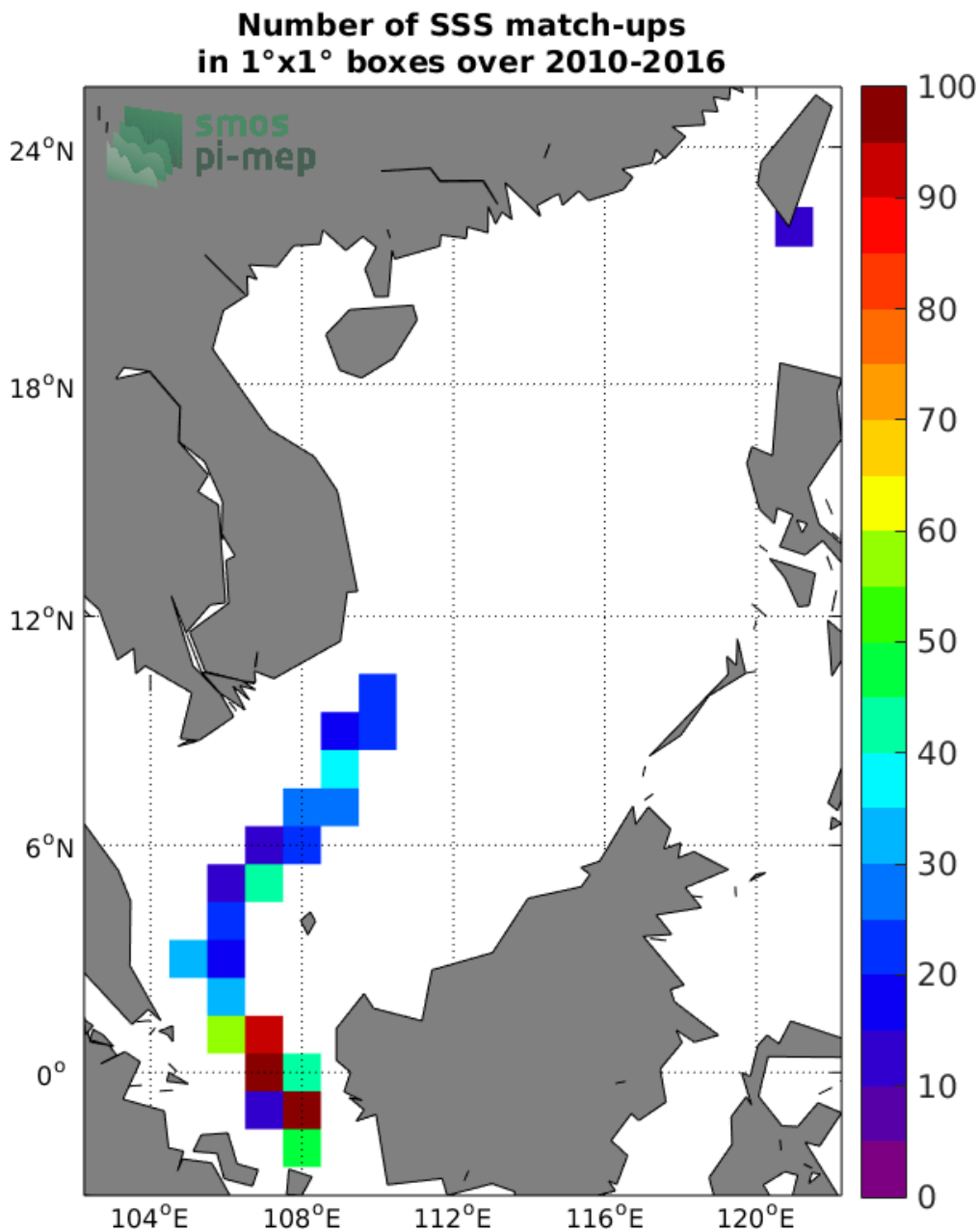
Figure 4: Number of SSS match-ups between TSG (LEGOS-DM) SSS and the SMOS SSS L2 v662 (ESA) SSS product for the South China Sea Pi-MEP region over 1°x1° boxes and for the full satellite product period.
