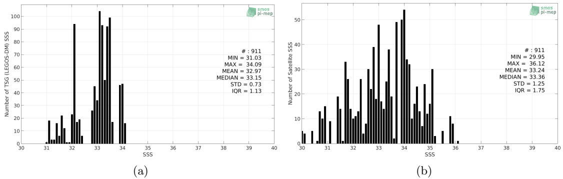
Figure 2: Histograms of SSS from TSG (LEGOS-DM) (a) and SMOS SSS L2 v662 (ESA) (b) considering all match-up pairs per bins of 0.1 over the South China Sea Pi-MEP region and for the full satellite product period.
