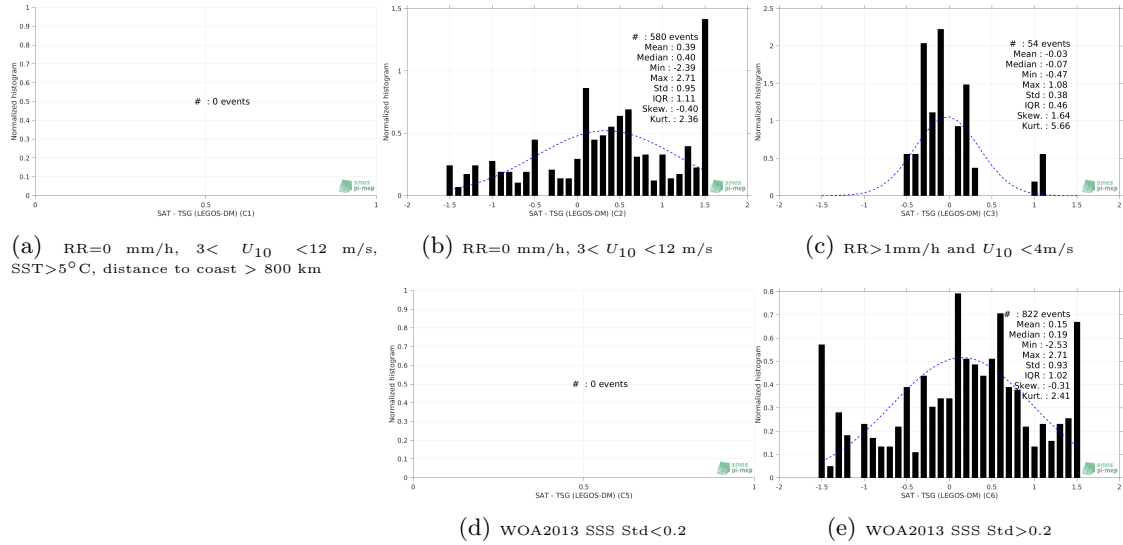
Figure 13: Normalized histogram of \Delta\text{SSS} (SMOS SSS L2 v662 (ESA) - TSG (LEGOS-DM)) for 5 different subdatasets corresponding to: RR=0 mm/h, 3 < U_{10} < 12 m/s, SST > 5^\circ\text{C} , distance to coast > 800 km (a), RR=0 mm/h, 3 < U_{10} < 12 m/s (b), RR > 1\text{mm/h} and U_{10} < 4\text{m/s} (c), WOA2013 SSS Std < 0.2 (d), WOA2013 SSS Std > 0.2 (e).
