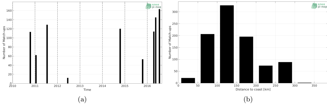
Figure 1: Number of match-ups between TSG (LEGOS-DM) and SMOS SSS L2 v662 (ESA) SSS as a function of time (a) and as function of the distance to coast (b) over the South China Sea Pi-MEP region and for the full satellite product period.
