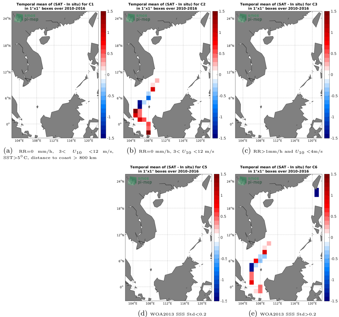
Figure 12: Temporal mean gridded over spatial boxes of size 1°x1° of \Delta SSS (SMOS SSS L2 v662 (ESA) - TSG (LEGOS-DM)) for 5 different subdatasets corresponding to: RR=0 mm/h, 3 < U_{10} < 12 m/s, SST > 5°C, distance to coast > 800 km (a), RR=0 mm/h, 3 < U_{10} < 12 m/s (b), RR > 1mm/h and U_{10} < 4 m/s (c), WOA2013 SSS Std < 0.2 (d), WOA2013 SSS Std > 0.2 (e).
