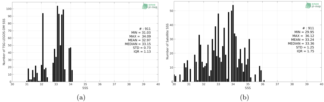
Figure 2: Histograms of SSS from TSG-LEGOS-DM (a) and SMOS L2 v662 (ESA) (b) considering all match-up pairs per bins of 0.1 over the South China Sea Pi-MEP region and for the full satellite product period.
