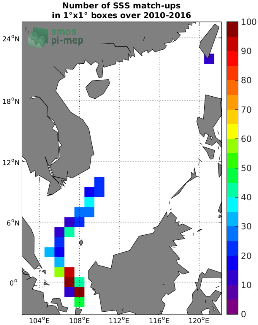
Figure 4: Number of SSS match-ups between TSG-LEGOS-DM SSS and the SMOS L2 v662 (ESA) SSS product for the South China Sea Pi-MEP region over 1°x1° boxes and for the full satellite product period.
