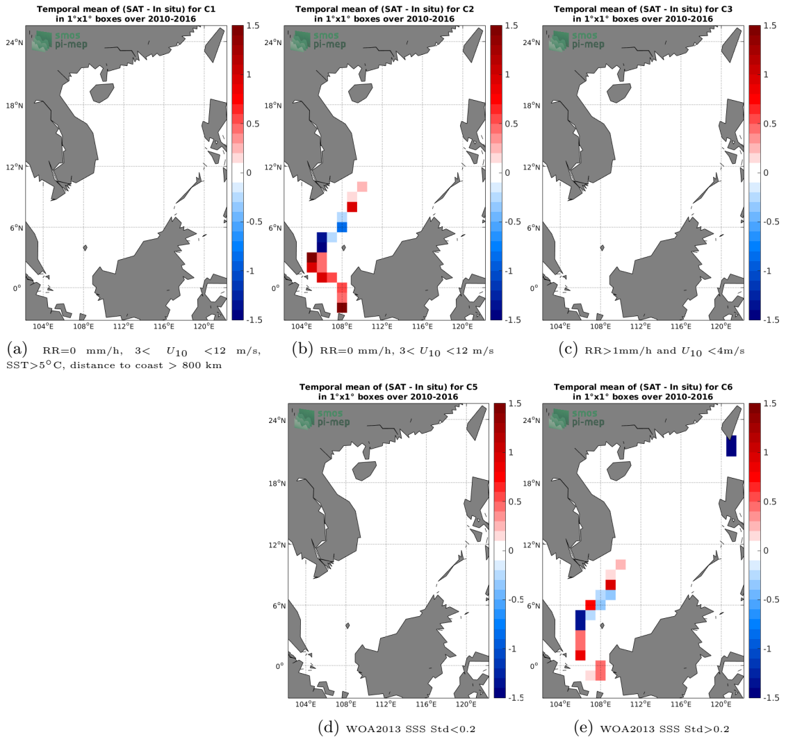
Figure 12: Temporal mean gridded over spatial boxes of size 1^\circ \times 1^\circ of \Delta SSS (SMOS L2 v662 (ESA) - TSG-LEGOS-DM) for 5 different subdatasets corresponding to:RR=0 mm/h, 3 < U_{10} < 12 m/s, SST > 5°C, distance to coast > 800 km (a), RR=0 mm/h, 3 < U_{10} < 12 m/s (b), RR > 1mm/h and U_{10} < 4 m/s (c), WOA2013 SSS Std < 0.2 (d), WOA2013 SSS Std > 0.2 (e).
