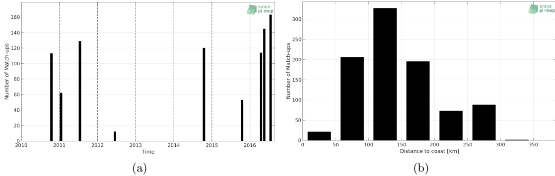
Figure 1: Number of match-ups between TSG-LEGOS-DM and SMOS L2 v662 (ESA) SSS as a function of time (a) and as function of the distance to coast (b) over the South China Sea Pi-MEP region and for the full satellite product period.
