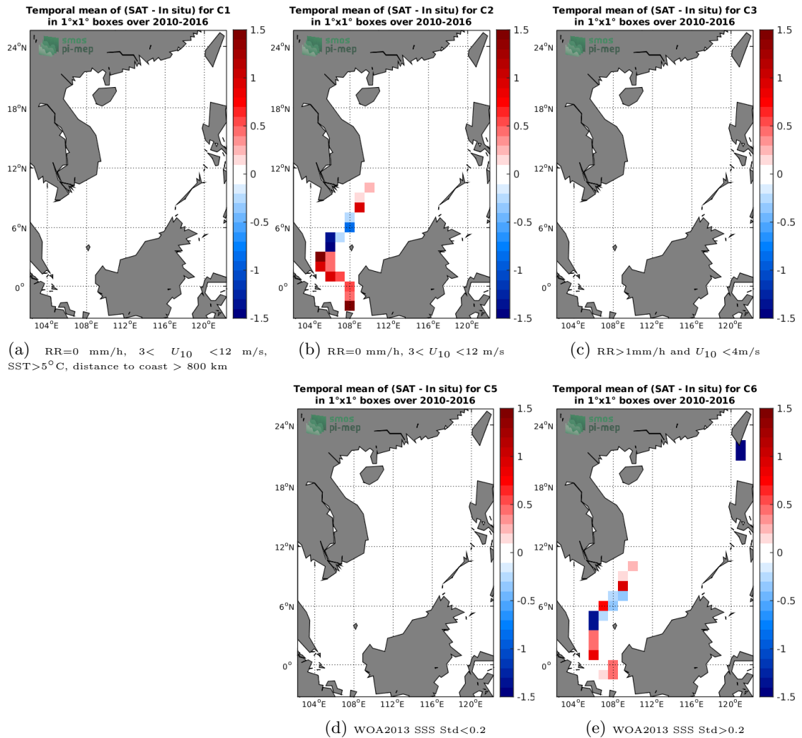
Figure 12: Temporal mean gridded over spatial boxes of size 1^\circ \times 1^\circ of \Delta SSS (SMOS-L2-DPGS-v662 - TSG-LEGOS-DM) for 5 different subdatasets corresponding to:RR=0 mm/h, 3 < U_{10} < 12 m/s, SST >5^\circ C, distance to coast > 800 km (a), RR=0 mm/h, 3 < U_{10} < 12 m/s (b), RR >1 mm/h and U_{10} < 4 m/s (c), WOA2013 SSS Std <0.2 (d), WOA2013 SSS Std >0.2 (e).
