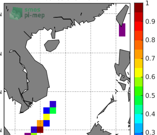
Temporal STD of (Sat - TSG-LEGOS-DM) in 1°x1° boxes over 2010-2016
