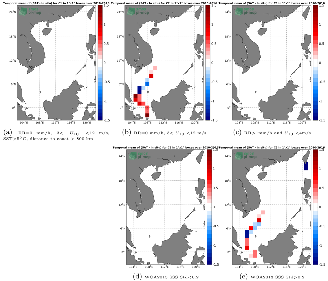
Figure 12: Temporal mean gridded over spatial boxes of size 1^\circ \times 1^\circ of \Delta SSS (SMOS-L2-DPGS-v662 - TSG-LEGOS-DM) for 5 different subdatasets corresponding to:RR=0 mm/h, 3 < U_{10} < 12 m/s, SST >5^\circ C, distance to coast > 800 km (a), RR=0 mm/h, 3 < U_{10} < 12 m/s (b), RR >1 mm/h and U_{10} < 4 m/s (c), WOA2013 SSS Std <0.2 (d), WOA2013 SSS Std >0.2 (e).
