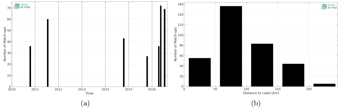
Figure 1: Number of match-ups between TSG-LEGOS-DM and SMOS-L2-DPGS-v662 SSS as a function of time (a) and as function of the distance to coast (b) over the South China Sea Pi-MEP region and for the full satellite product period.
