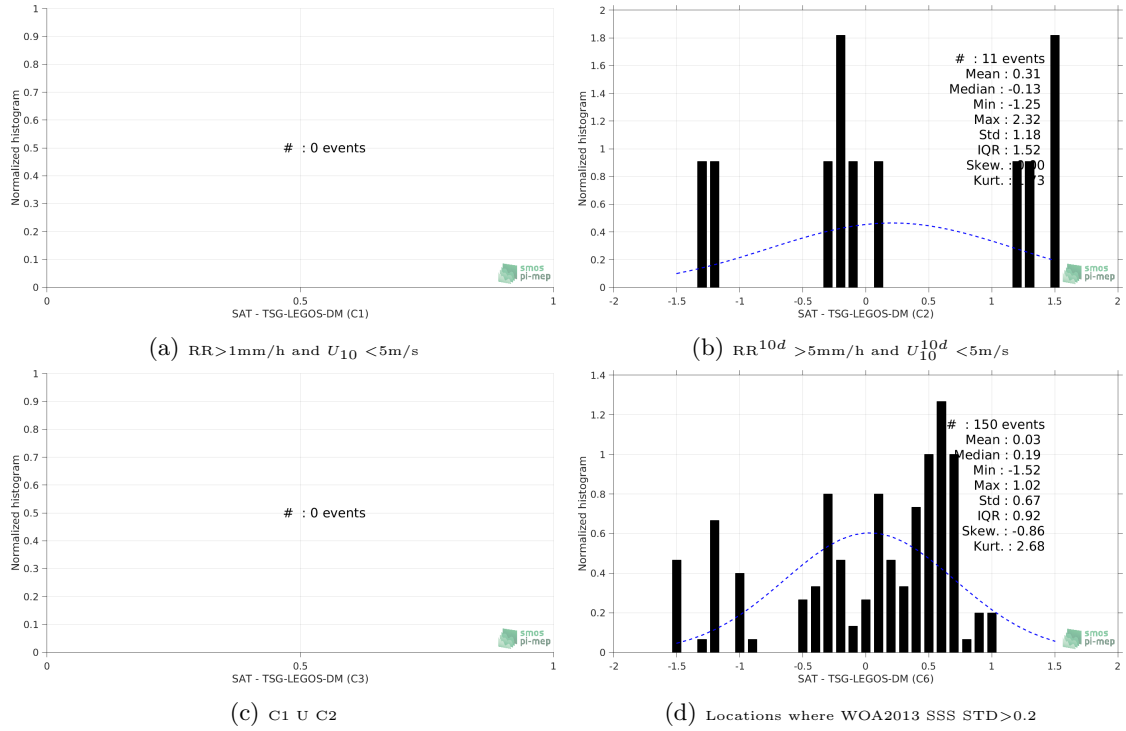
Figure 13: Normalized histogram of \Delta\text{SSS} (SMOS-L2-DPGS-v662 - TSG-LEGOS-DM) for 6 different subdatasets corresponding to: RR > 1\text{mm/h} and U_{10} < 5\text{m/s} (a), RR^{10d} > 5\text{mm/h} and U_{10}^{10d} < 5\text{m/s} (b), C1 U C2 (c), Locations where WOA2013 SSS STD > 0.2 (d).
