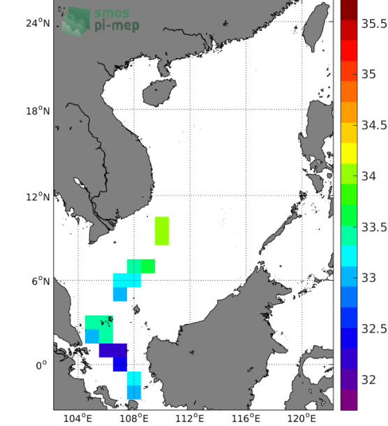
(c) MEAN(TSG-LEGOS-DM SSS)
