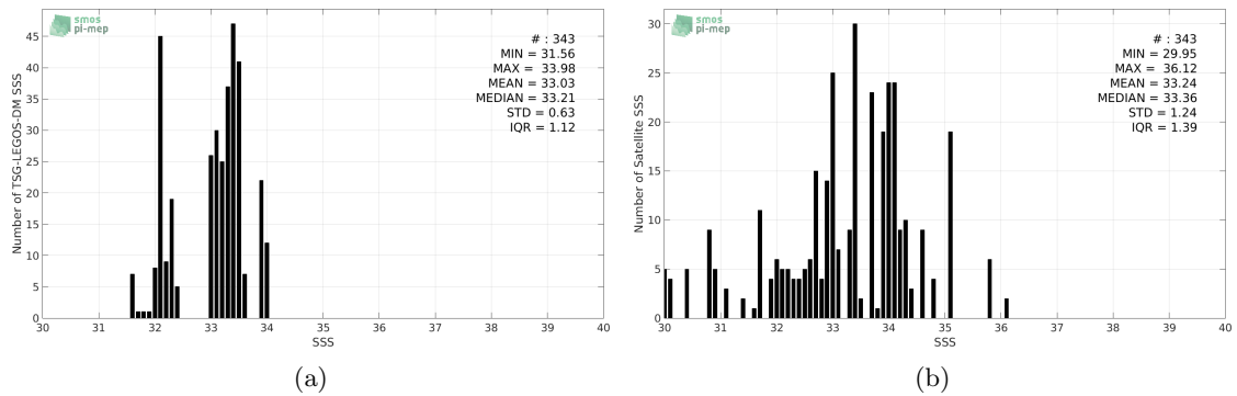
Figure 2: Histograms of SSS from TSG-LEGOS-DM (a) and SMOS-L2-DPGS-v662 (b) considering all match-up pairs per bins of 0.1 over the South China Sea Pi-MEP region and for the full satellite product period.
