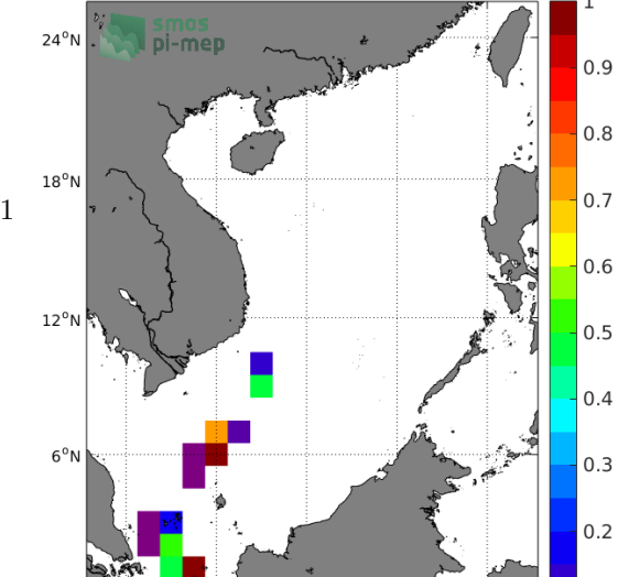
Temporal STD of (Sat-TSG-LEGOS-DM) in 1°x1° boxes over 2010-2016
