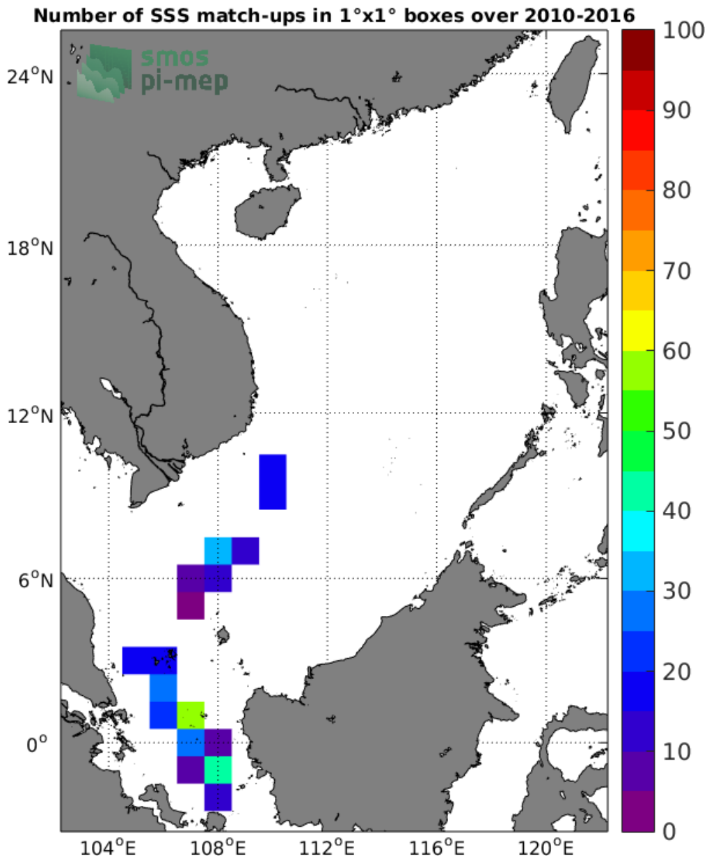
Figure 4: Number of SSS match-ups between TSG-LEGOS-DM SSS and the SMOS-L2-DPGS-v662 SSS product for the South China Sea Pi-MEP region over 1°x1° boxes and for the full satellite product period.
