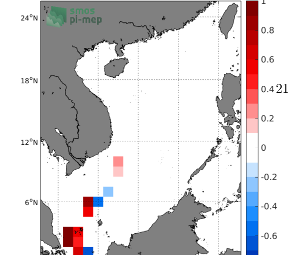
Temporal mean of (Sat-TSG-LEGOS-DM) in 1°x1° boxes over 2010-2016
