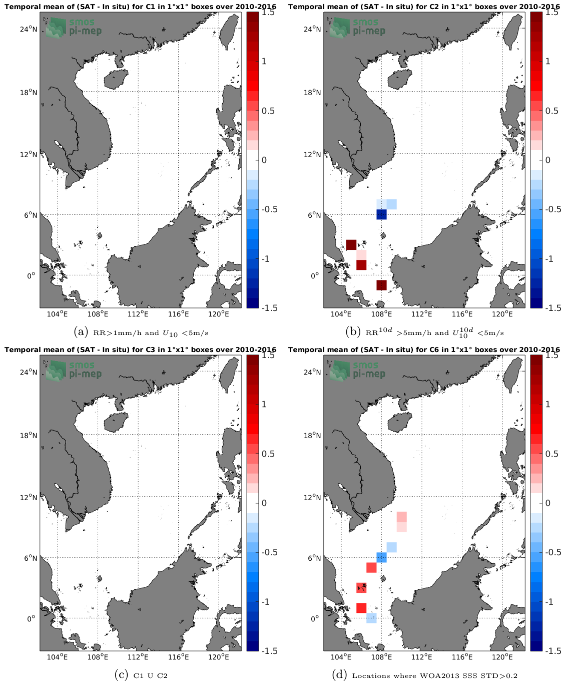
Figure 12: Temporal mean gridded over spatial boxes of size 1°x1° of \Delta\text{SSS} (SMOS-L2-DPGS-v662 - TSG-LEGOS-DM) for 4 different subdatasets corresponding to: RR > 1\text{mm/h} and U_{10} < 5\text{m/s} (a), RR^{10d} > 5\text{mm/h} and U_{10}^{10d} < 5\text{m/s} (b), C1 U C2 (c), Locations where WOA2013 SSS STD > 0.2 (d).
