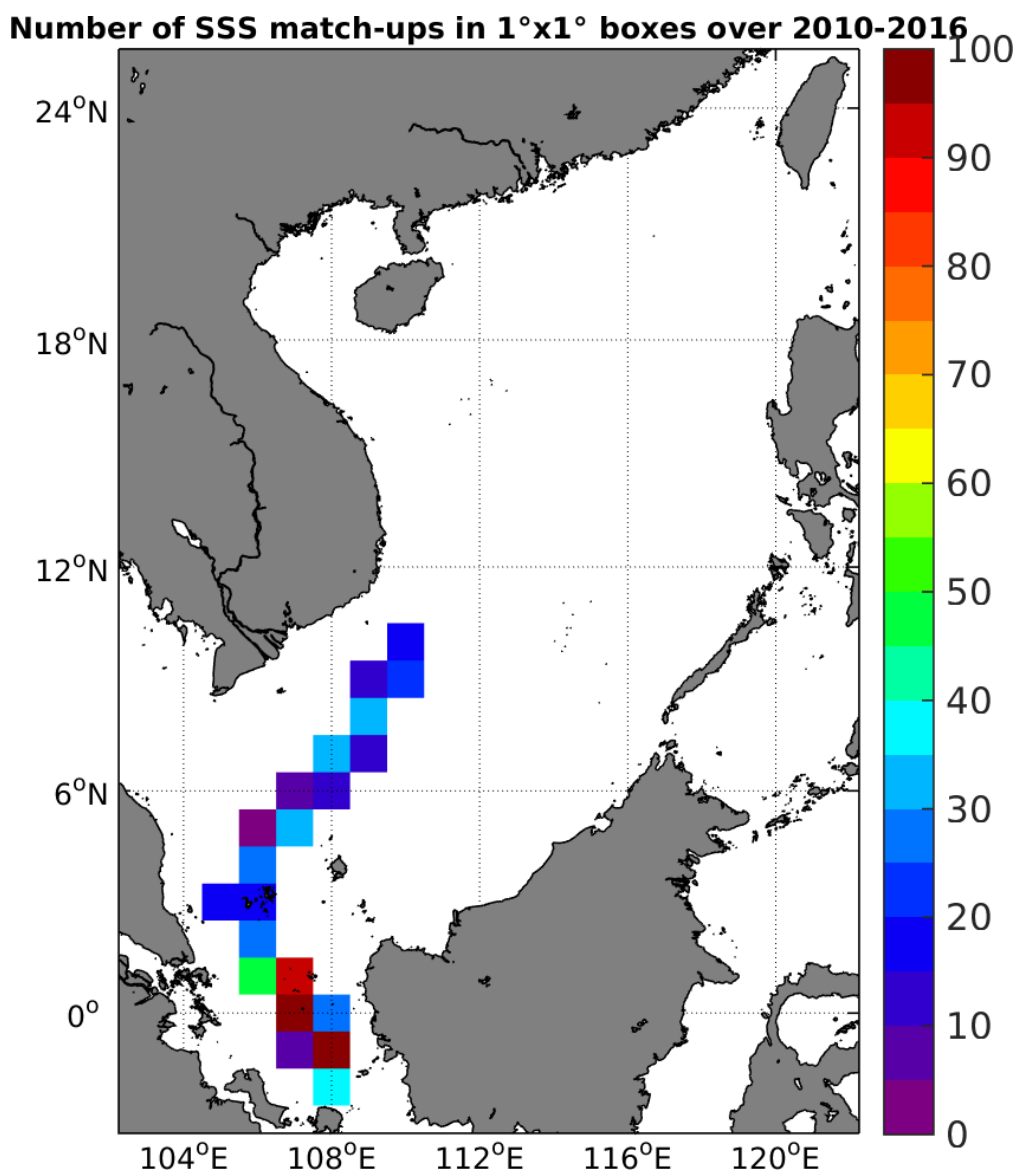
Figure 4: Number of SSS match-ups between TSG-LEGOS-DM SSS and the SMOS-L2-DPGS-v662 SSS product for the South China Sea Pi-MEP region over 1°x1° boxes and for the full satellite product period.
