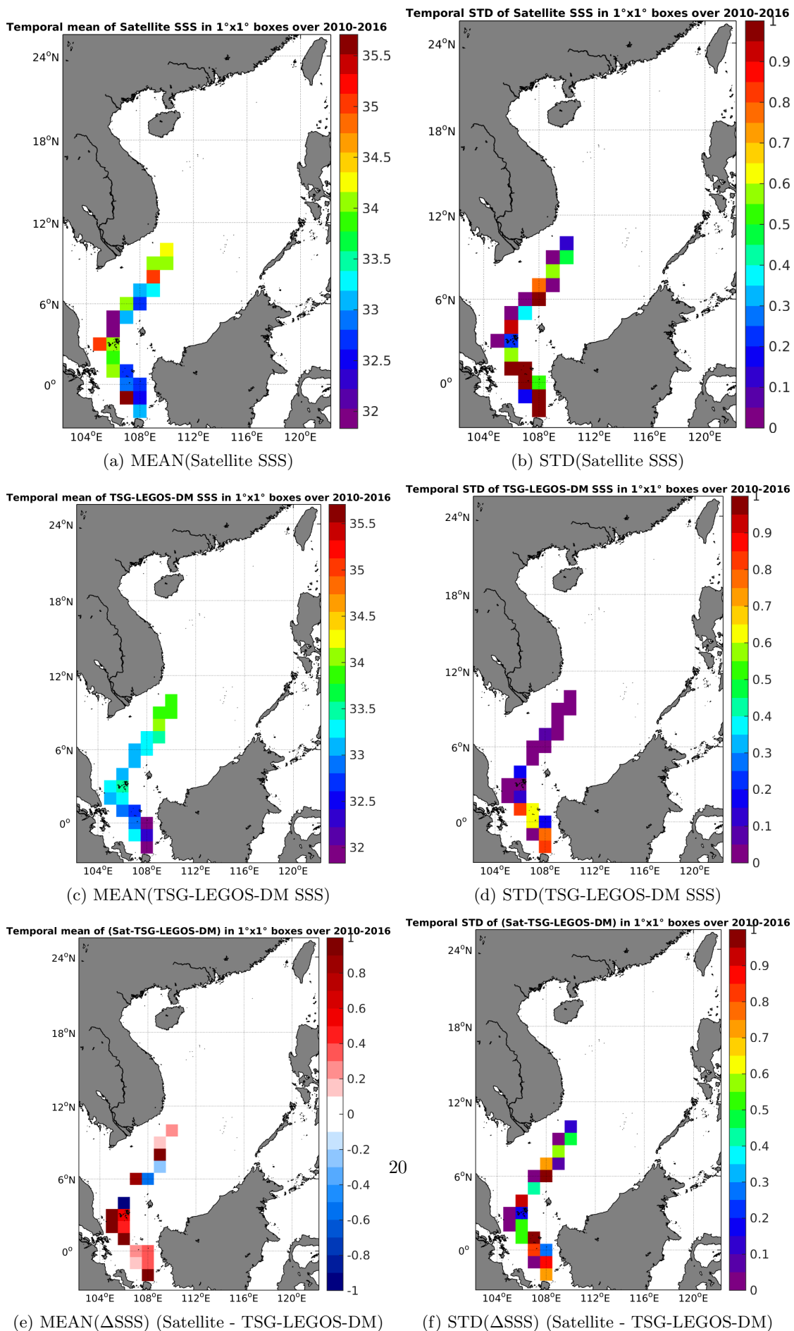
Figure 6: Temporal mean (left) and STD (right) of SSS from SMOS-L2-DPGS-v662 (top), TSG-LEGOS-DM (middle), and of \Delta SSS (Satellite - TSG-LEGOS-DM). Only match-up pairs are used to generate these maps.
