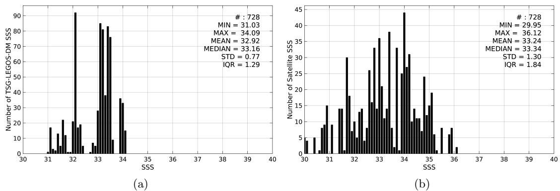
Figure 2: Histograms of SSS from TSG-LEGOS-DM (a) and SMOS-L2-DPGS-v662 (b) considering all match-up pairs per bins of 0.1 over the South China Sea Pi-MEP region and for the full satellite product period.
