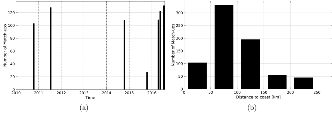
Figure 1: Number of match-ups between TSG-LEGOS-DM and SMOS-L2-DPGS-v662 SSS as a function of time (a) and as function of the distance to coast (b) over the South China Sea Pi-MEP region and for the full satellite product period.
