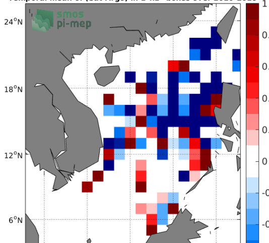
Temporal mean of (Sat-Argo) in 1°x1° boxes over 2010-2019
