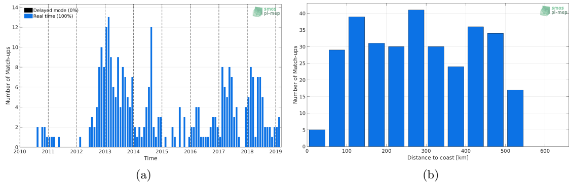
Figure 1: Number of match-ups between Argo and SMOS-L2-DPGS-v662 SSS as a function of time (a) and as function of the distance to coast (b) over the South China Sea Pi-MEP region and for the full satellite product period.
