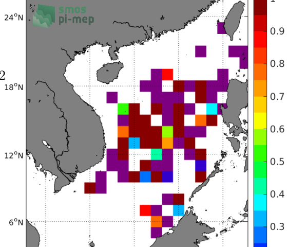
Temporal STD of (Sat-Argo) in 1°x1° boxes over 2011-2018
