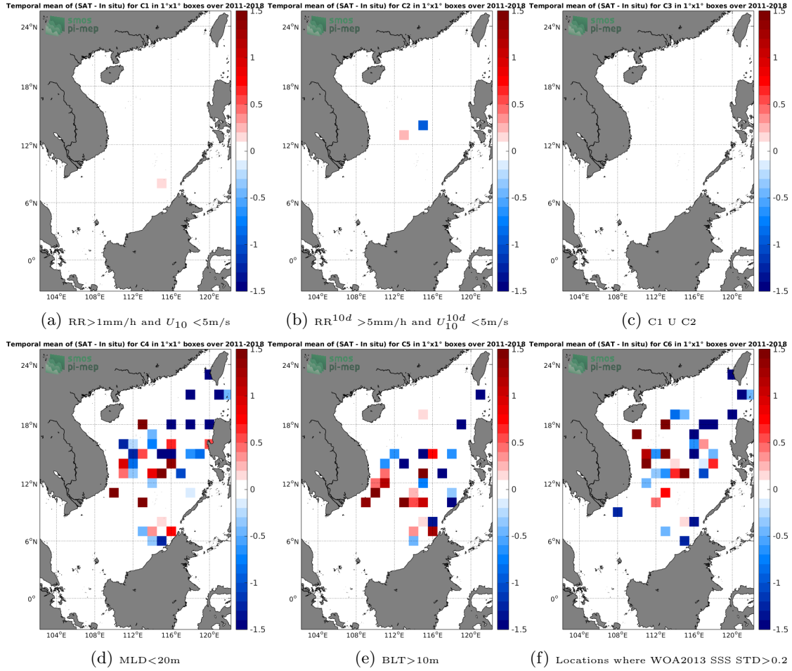
Figure 12: Temporal mean gridded over spatial boxes of size 1°x1° of \Delta SSS (SMOS-L2-DPGS-v662 - Argo) for 6 different subdatasets corresponding to:RR>1mm/h and U_{10} < 5m/s (a), RR^{10d} > 5mm/h and U_{10}^{10d} < 5m/s (b), C1 U C2 (c),MLD<20m (d),BLT>10m (e),Locations where WOA2013 SSS STD>0.2 (f).
