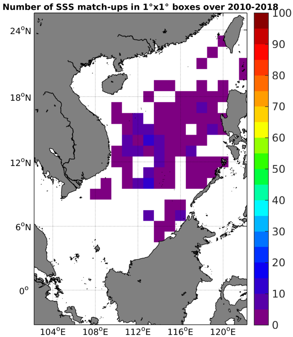
Figure 4: Number of SSS match-ups between Argo SSS and the SMOS-L2-DPGS-v662 SSS product for the South China Sea Pi-MEP region over 1°x1° boxes and for the full satellite product period.
