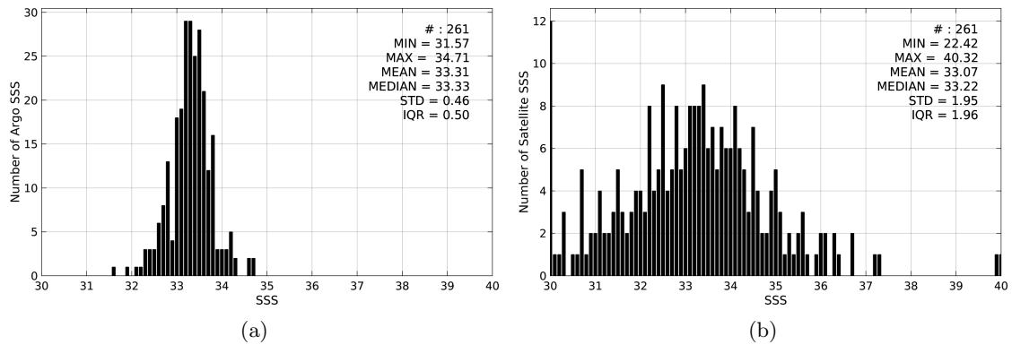
Figure 2: Histograms of SSS from Argo (a) and SMOS-L2-DPGS-v662 (b) considering all match-up pairs per bins of 0.1 over the South China Sea Pi-MEP region and for the full satellite product period.
