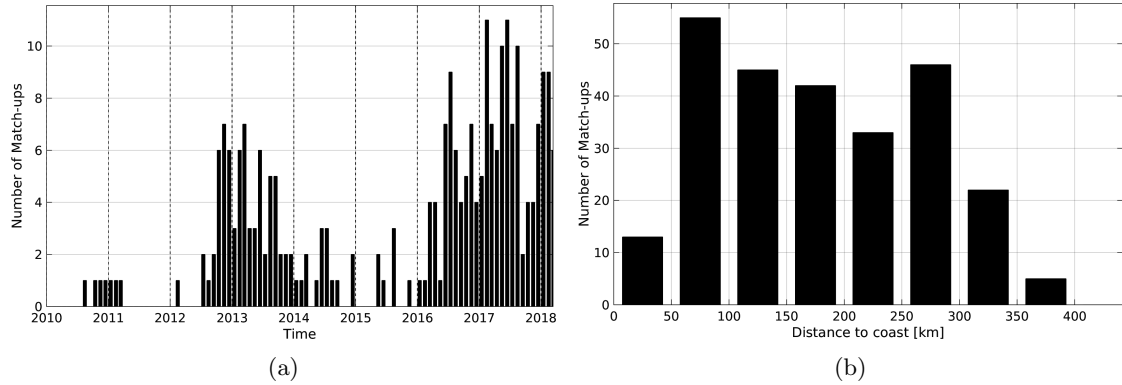
Figure 1: Number of match-ups between Argo and SMOS-L2-DPGS-v662 SSS as a function of time (a) and as function of the distance to coast (b) over the South China Sea Pi-MEP region and for the full satellite product period.
