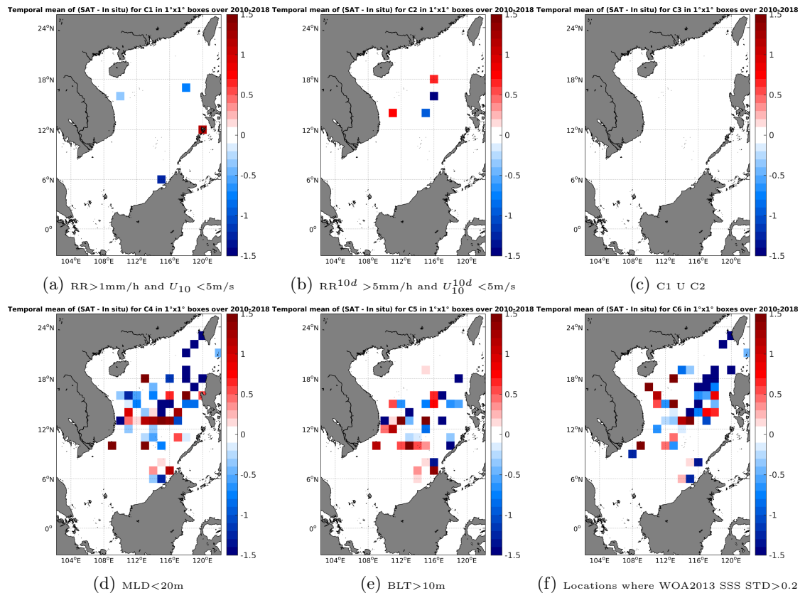
Figure 12: Temporal mean gridded over spatial boxes of size 1^\circ \times 1^\circ of \Delta\text{SSS} (SMOS-L2-DPGS-v662 - Argo) for 6 different subdatasets corresponding to: \text{RR} > 1\text{mm/h} and U_{10} < 5\text{m/s} (a), \text{RR}^{10d} > 5\text{mm/h} and U_{10}^{10d} < 5\text{m/s} (b), C1 U C2 (c), \text{MLD} < 20\text{m} (d), \text{BLT} > 10\text{m} (e), Locations where WOA2013 SSS STD > 0.2 (f).
