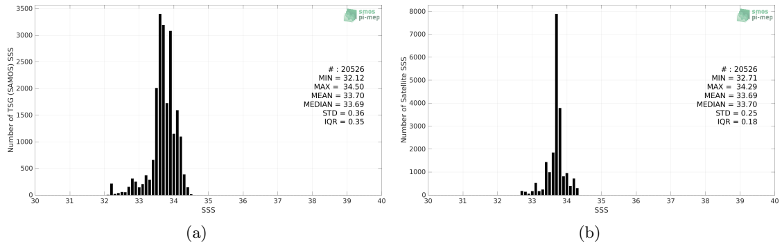
Figure 2: Histograms of SSS from TSG (SAMOS) (a) and SMAP SSS L4 OI v1 - 7 Days (IPRC) (b) considering all match-up pairs per bins of 0.1 over the South China Sea Pi-MEP region and for the full satellite product period.
