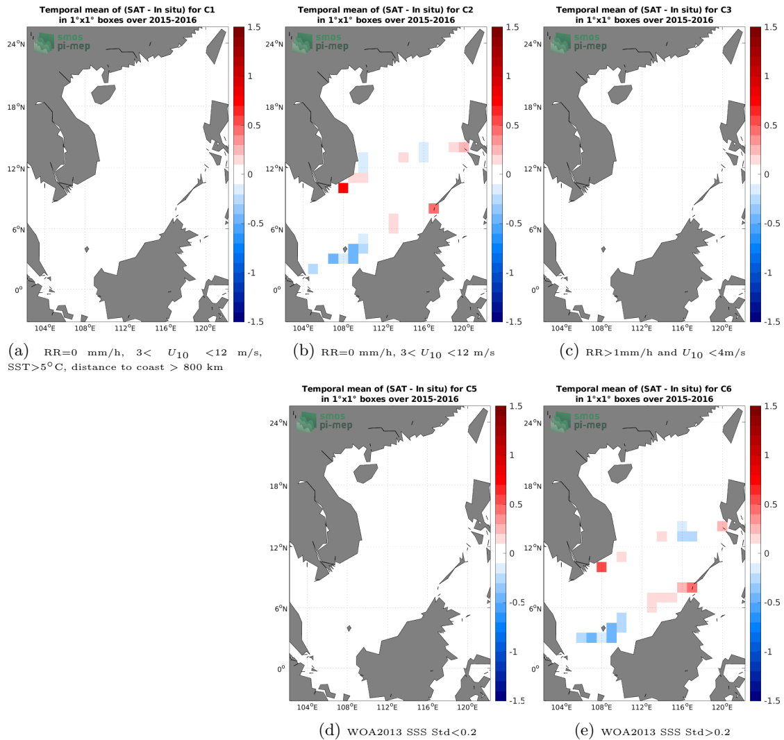
Figure 12: Temporal mean gridded over spatial boxes of size 1^\circ \times 1^\circ of \Delta SSS (SMAP SSS L4 OI v1 - 7 Days (IPRC) - TSG (SAMOS)) for 5 different subdatasets corresponding to:RR=0 mm/h, 3 < U_{10} < 12 m/s, SST>5°C, distance to coast > 800 km (a), RR=0 mm/h, 3 < U_{10} < 12 m/s (b), RR>1mm/h and U_{10} < 4 m/s (c), WOA2013 SSS Std<0.2 (d), WOA2013 SSS Std>0.2 (e).
