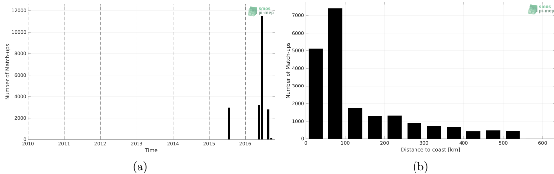
Figure 1: Number of match-ups between TSG (SAMOS) and SMAP SSS L4 OI v1 - 7 Days (IPRC) SSS as a function of time (a) and as function of the distance to coast (b) over the South China Sea Pi-MEP region and for the full satellite product period.
