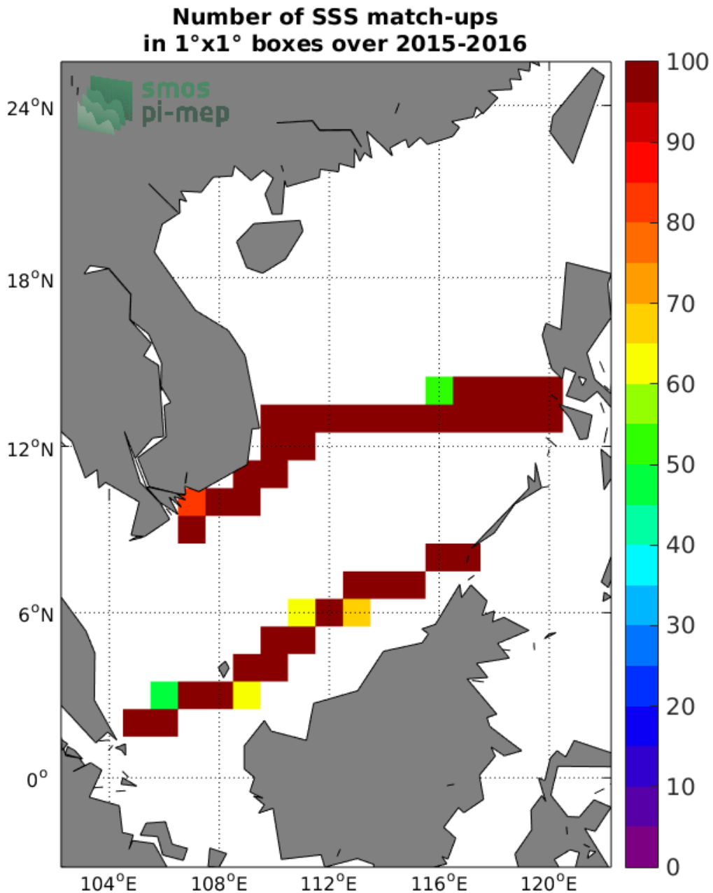
Figure 4: Number of SSS match-ups between TSG (SAMOS) SSS and the SMAP SSS L4 OI v1 - 7 Days (IPRC) SSS product for the South China Sea Pi-MEP region over 1°x1° boxes and for the full satellite product period.
