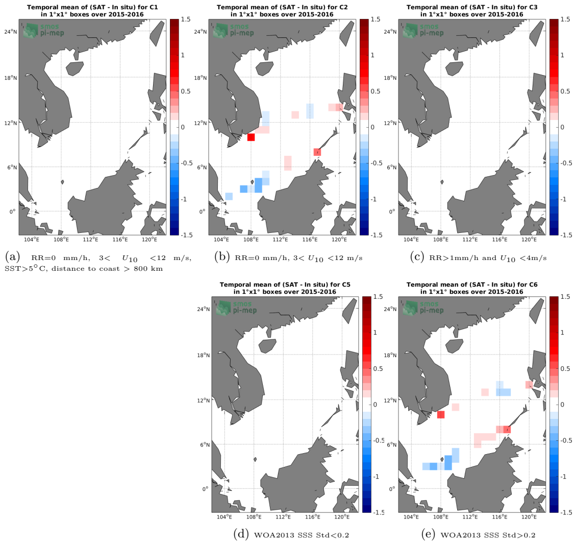
Figure 12: Temporal mean gridded over spatial boxes of size 1°x1° of \Delta SSS (SMAP SSS L4 OI v1 - 7day (IPRC) - TSG (SAMOS)) for 5 different subdatasets corresponding to: RR=0 mm/h, 3 < U_{10} < 12 m/s, SST > 5°C, distance to coast > 800 km (a), RR=0 mm/h, 3 < U_{10} < 12 m/s (b), RR > 1mm/h and U_{10} < 4m/s (c), WOA2013 SSS Std < 0.2 (d), WOA2013 SSS Std > 0.2 (e).
