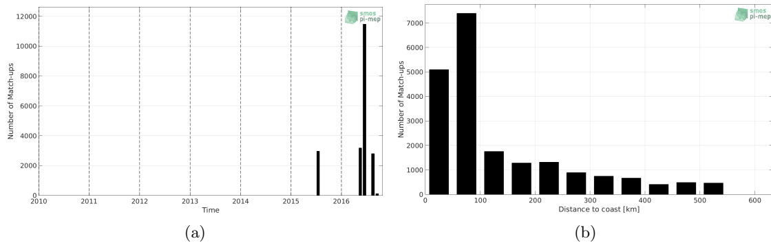
Figure 1: Number of match-ups between TSG (SAMOS) and SMAP SSS L4 OI v1 - 7day (IPRC) SSS as a function of time (a) and as function of the distance to coast (b) over the South China Sea Pi-MEP region and for the full satellite product period.
