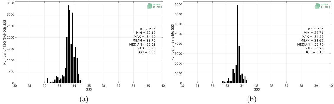
Figure 2: Histograms of SSS from TSG (SAMOS) (a) and SMAP SSS L4 OI v1 - 7day (IPRC) (b) considering all match-up pairs per bins of 0.1 over the South China Sea Pi-MEP region and for the full satellite product period.
