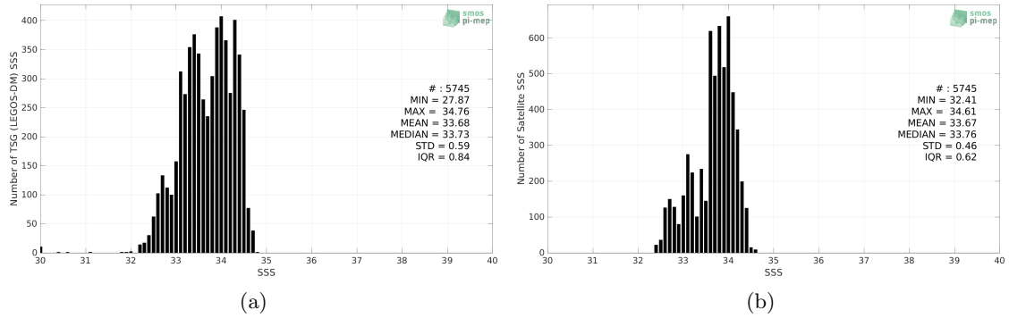
Figure 2: Histograms of SSS from TSG (LEGOS-DM) (a) and SMAP SSS L4 OI v1 - 7 Days (IPRC) (b) considering all match-up pairs per bins of 0.1 over the South China Sea Pi-MEP region and for the full satellite product period.
