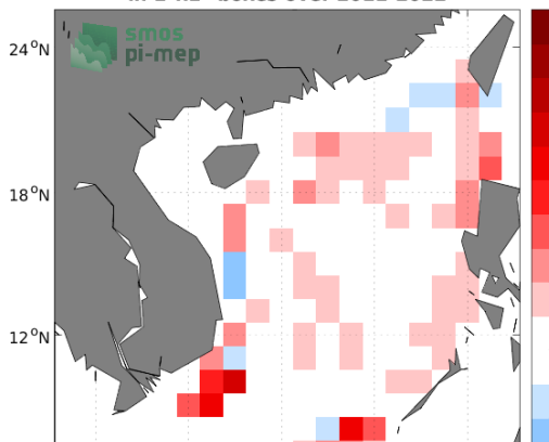
Temporal mean of (Sat - Argo) in 1°x1° boxes over 2011-2022
