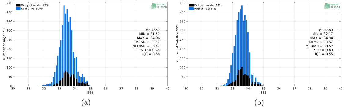
Figure 2: Histograms of SSS from Argo (a) and SMAP SSS L4 OI v1 - 7 Days (IPRC) (b) considering all match-up pairs per bins of 0.1 over the South China Sea Pi-MEP region and for the full satellite product period.
