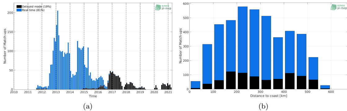
Figure 1: Number of match-ups between Argo and SMAP SSS L4 OI v1 - 7 Days (IPRC) SSS as a function of time (a) and as function of the distance to coast (b) over the South China Sea Pi-MEP region and for the full satellite product period.
