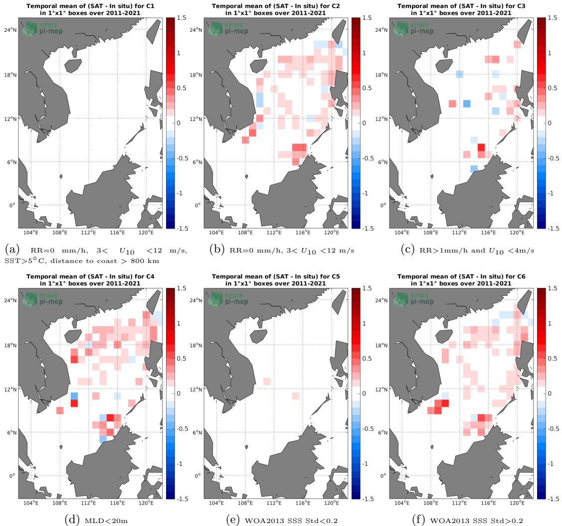
Figure 12: Temporal mean gridded over spatial boxes of size 1°x1° of \Delta SSS (SMAP SSS L4 OI v1 - 7day (IPRC) - Argo) for 6 different subdatasets corresponding to:RR=0 mm/h, 3 < U_{10} < 12 m/s, SST>5°C, distance to coast > 800 km (a), RR=0 mm/h, 3 < U_{10} < 12 m/s (b), RR>1mm/h and U_{10} < 4 m/s (c),MLD<20m (d),WOA2013 SSS Std<0.2 (e),WOA2013 SSS Std>0.2 (f).
