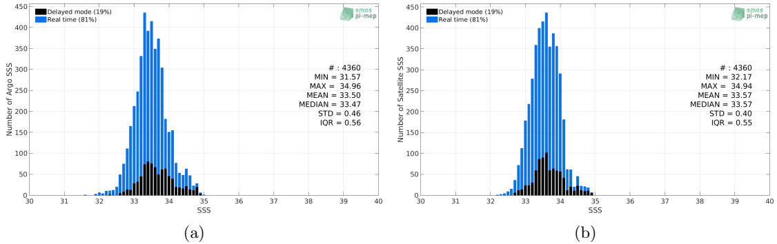
Figure 2: Histograms of SSS from Argo (a) and SMAP SSS L4 OI v1 - 7day (IPRC) (b) considering all match-up pairs per bins of 0.1 over the South China Sea Pi-MEP region and for the full satellite product period.
