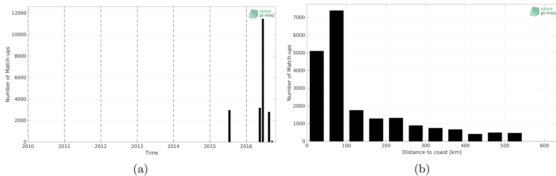
Figure 1: Number of match-ups between TSG (SAMOS) and SMAP SSS L4 OI v1 - Monthly (IPRC) SSS as a function of time (a) and as function of the distance to coast (b) over the South China Sea Pi-MEP region and for the full satellite product period.
