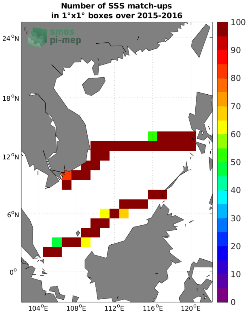
Figure 4: Number of SSS match-ups between TSG (SAMOS) SSS and the SMAP SSS L4 OI v1 - Monthly (IPRC) SSS product for the South China Sea Pi-MEP region over 1°x1° boxes and for the full satellite product period.
