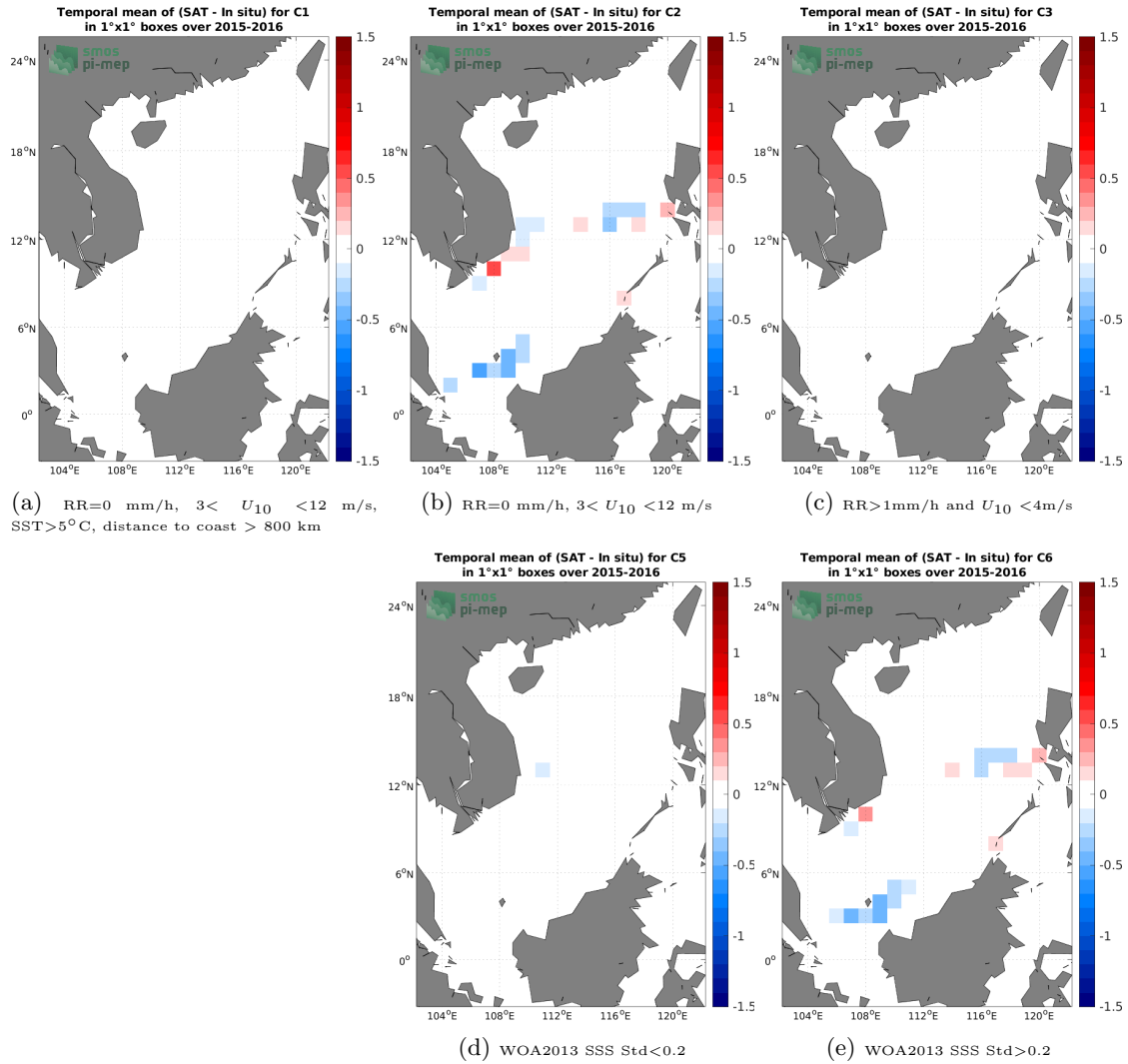
Figure 12: Temporal mean gridded over spatial boxes of size 1^\circ \times 1^\circ of \Delta SSS (SMAP SSS L4 OI v1 - Monthly (IPRC) - TSG (SAMOS)) for 5 different subdatasets corresponding to: RR=0 mm/h, 3 < U_{10} < 12 m/s, SST>5°C, distance to coast > 800 km (a), RR=0 mm/h, 3 < U_{10} < 12 m/s (b), RR>1mm/h and U_{10} < 4 m/s (c), WOA2013 SSS Std<0.2 (d), WOA2013 SSS Std>0.2 (e).
