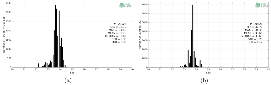
Figure 2: Histograms of SSS from TSG (SAMOS) (a) and SMAP SSS L4 OI v1 - Monthly (IPRC) (b) considering all match-up pairs per bins of 0.1 over the South China Sea Pi-MEP region and for the full satellite product period.
