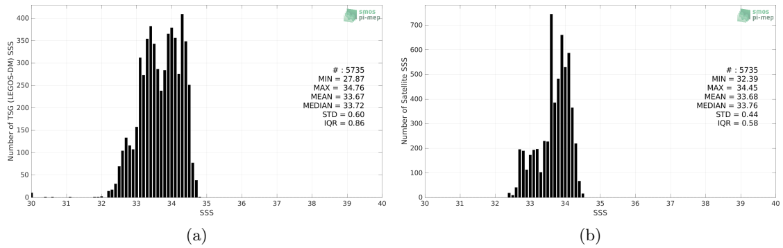
Figure 2: Histograms of SSS from TSG (LEGOS-DM) (a) and SMAP SSS L4 OI v1 - Monthly (IPRC) (b) considering all match-up pairs per bins of 0.1 over the South China Sea Pi-MEP region and for the full satellite product period.
