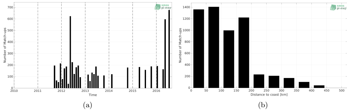
Figure 1: Number of match-ups between TSG (LEGOS-DM) and SMAP SSS L4 OI v1 - Monthly (IPRC) SSS as a function of time (a) and as function of the distance to coast (b) over the South China Sea Pi-MEP region and for the full satellite product period.
