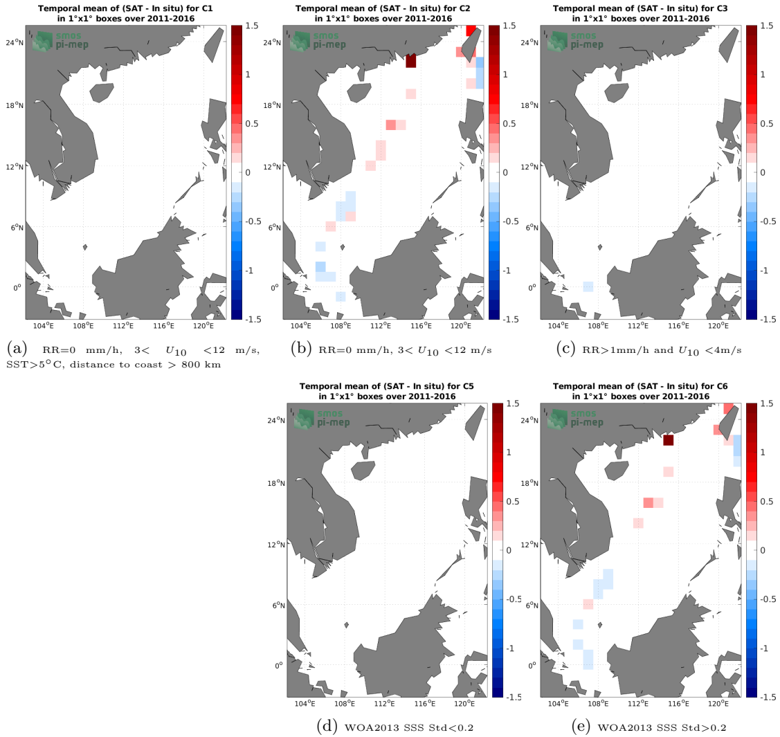
Figure 12: Temporal mean gridded over spatial boxes of size 1^\circ \times 1^\circ of \Delta SSS (SMAP SSS L4 OI v1 - Monthly (IPRC) - TSG (LEGOS-DM)) for 5 different subdatasets corresponding to: RR=0 mm/h, 3 < U_{10} < 12 m/s, SST > 5°C, distance to coast > 800 km (a), RR=0 mm/h, 3 < U_{10} < 12 m/s (b), RR > 1mm/h and U_{10} < 4 m/s (c), WOA2013 SSS Std < 0.2 (d), WOA2013 SSS Std > 0.2 (e).
