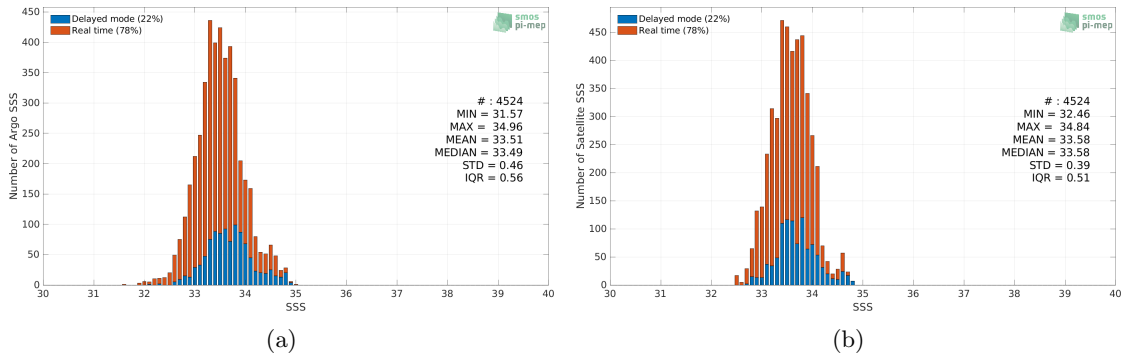
Figure 2: Histograms of SSS from Argo (a) and SMAP SSS L4 OI v1 - Monthly (IPRC) (b) considering all match-up pairs per bins of 0.1 over the South China Sea Pi-MEP region and for the full satellite product period.
