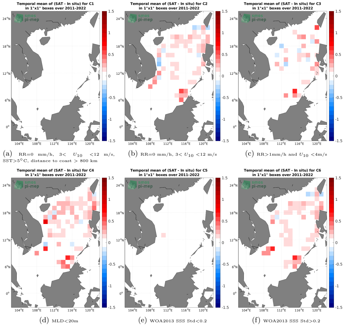
Figure 12: Temporal mean gridded over spatial boxes of size 1^\circ \times 1^\circ of \Delta\text{SSS} (SMAP SSS L4 OI v1 - Monthly (IPRC) - Argo) for 6 different subdatasets corresponding to: RR=0 mm/h, 3 < U_{10} < 12 m/s, SST > 5^\circ\text{C} , distance to coast > 800 km (a), RR=0 mm/h, 3 < U_{10} < 12 m/s (b), RR > 1 mm/h and U_{10} < 4 m/s (c), MLD < 20 m (d), WOA2013 SSS Std < 0.2 (e), WOA2013 SSS Std > 0.2 (f).
