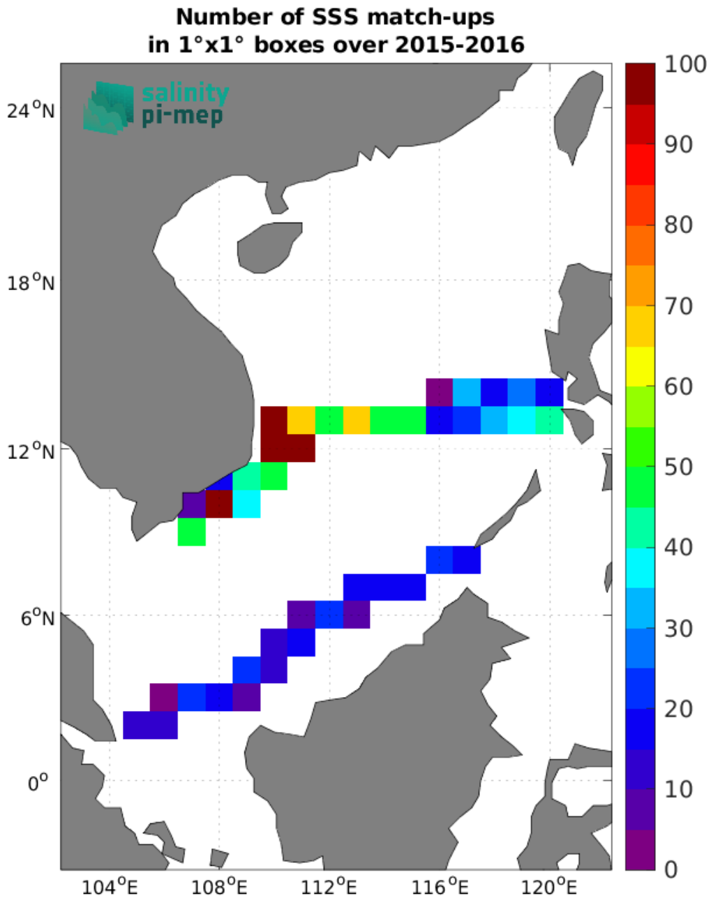
Figure 5: Number of SSS match-ups between TSG (SAMOS) SSS and the SMAP SSS L4 OI v3 - Monthly (ESR) SSS product for the South China Sea Pi-MEP region over 1°x1° boxes and for the full satellite product period.
