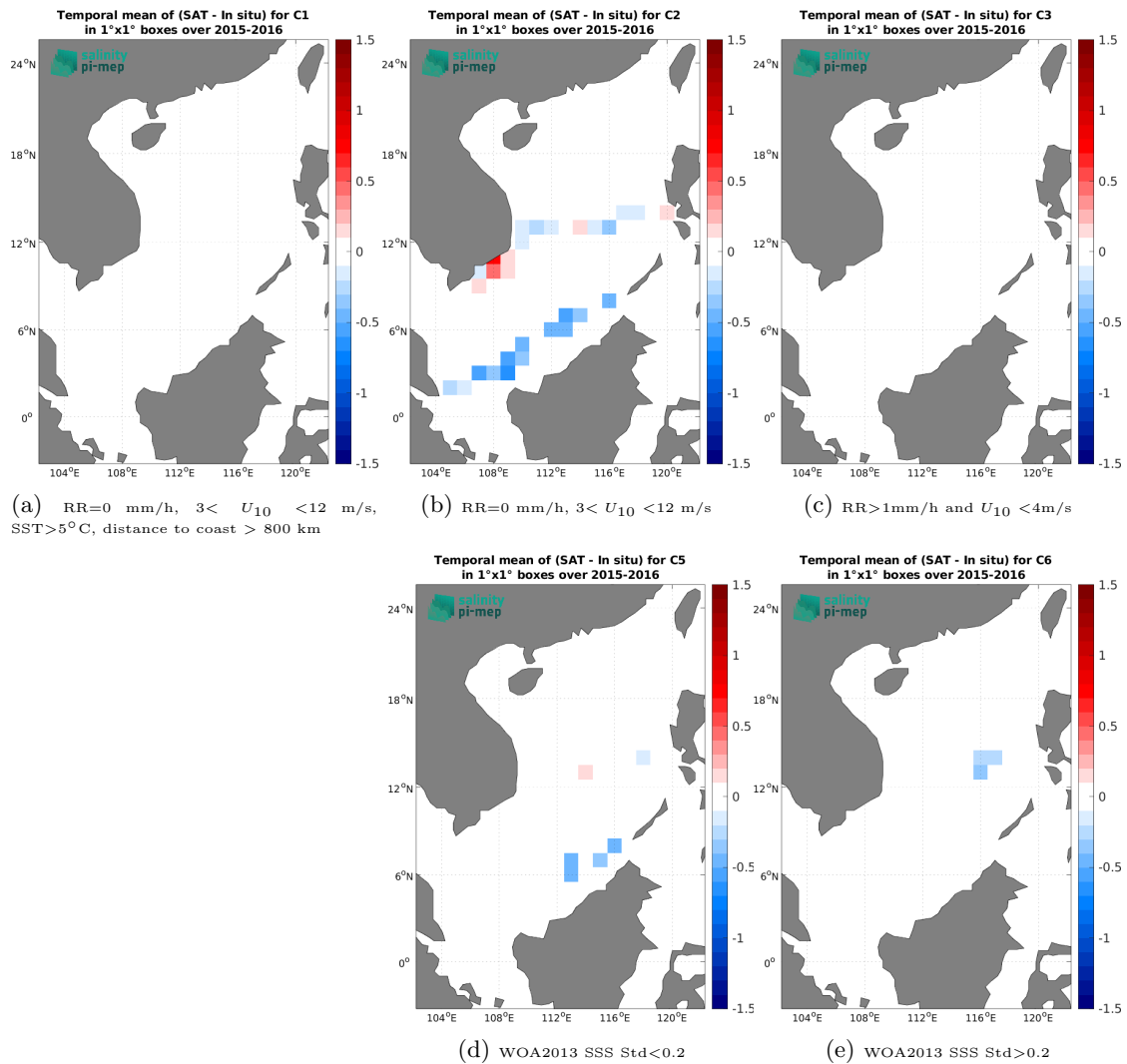
Figure 14: Temporal mean gridded over spatial boxes of size 1^\circ \times 1^\circ of \Delta\text{SSS} (SMAP SSS L4 OI v3 - Monthly (ESR) - TSG (SAMOS)) for 5 different subdatasets corresponding to: RR=0 mm/h, 3 < U_{10} < 12 m/s, SST > 5^\circ\text{C} , distance to coast > 800 km (a), RR=0 mm/h, 3 < U_{10} < 12 m/s (b), RR > 1 mm/h and U_{10} < 4 m/s (c), WOA2013 SSS Std < 0.2 (d), WOA2013 SSS Std > 0.2 (e).
