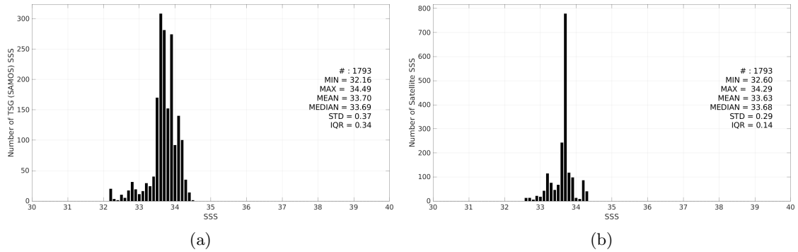
Figure 3: Histograms of SSS from TSG (SAMOS) (a) and SMAP SSS L4 OI v3 - Monthly (ESR) (b) considering all match-up pairs per bins of 0.1 over the South China Sea Pi-MEP region and for the full satellite product period.
