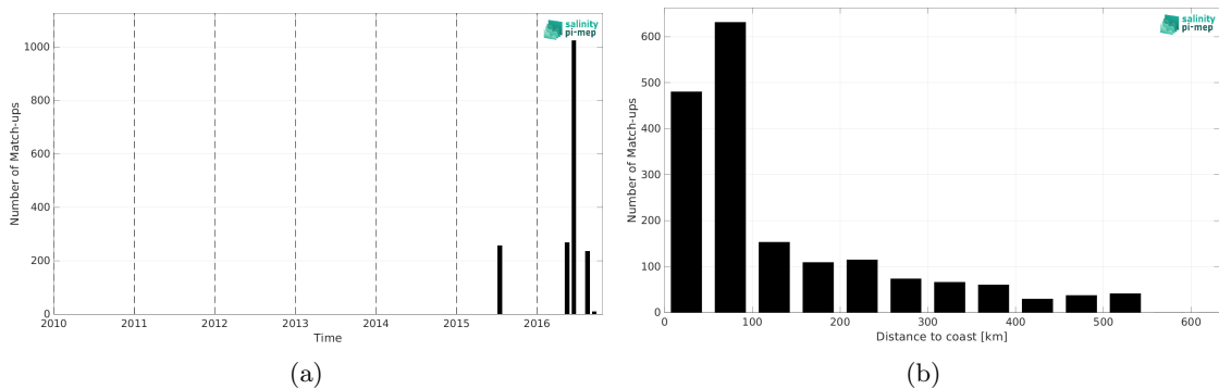
Figure 2: Number of match-ups between TSG (SAMOS) and SMAP SSS L4 OI v3 - Monthly (ESR) SSS as a function of time (a) and as function of the distance to coast (b) over the South China Sea Pi-MEP region and for the full satellite product period.
