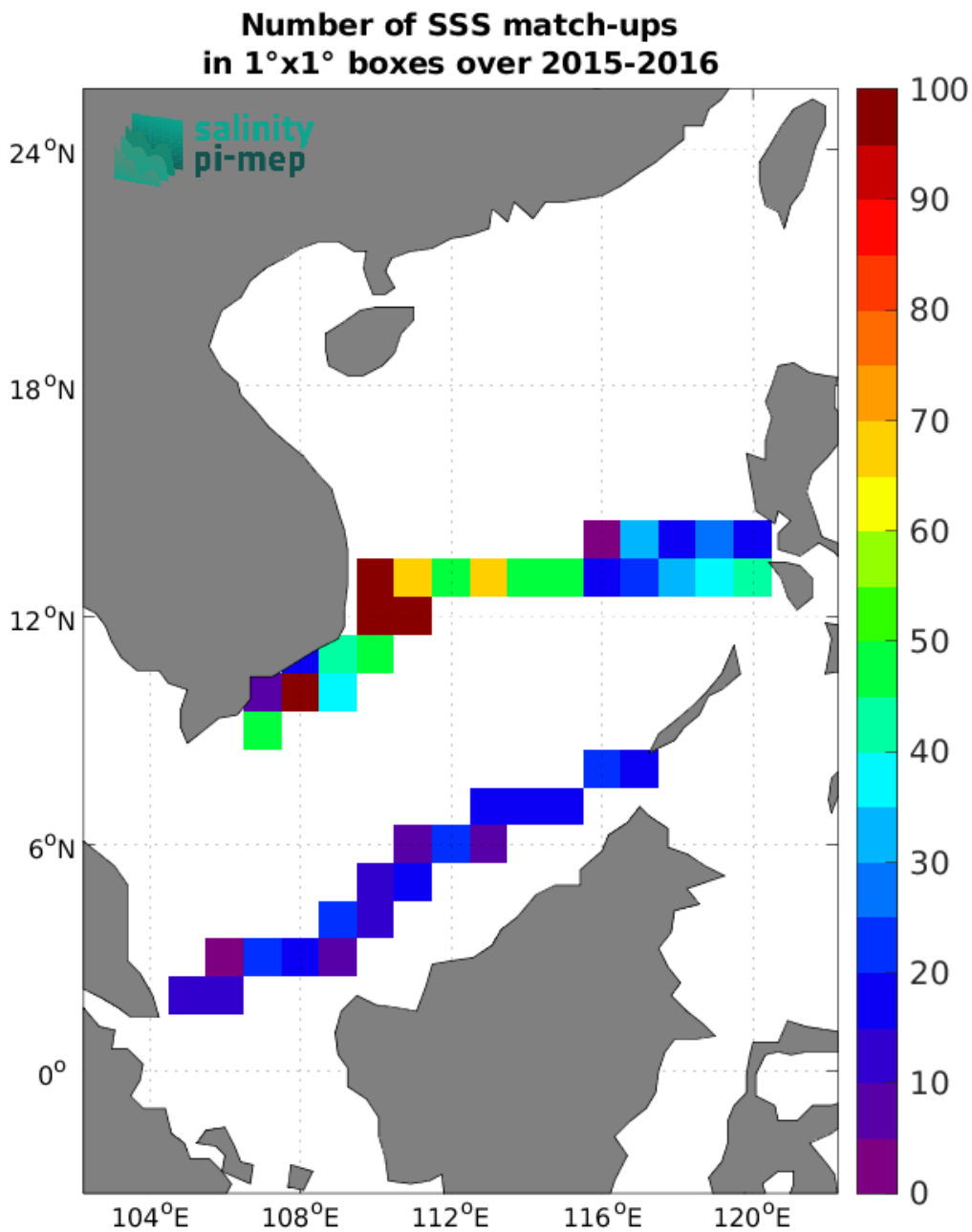
Figure 5: Number of SSS match-ups between TSG (SAMOS) SSS and the SMAP SSS L4 OI v3 - Monthly (ESR) SSS product for the South China Sea Pi-MEP region over 1^{\circ} \times 1^{\circ} boxes and for the full satellite product period.
