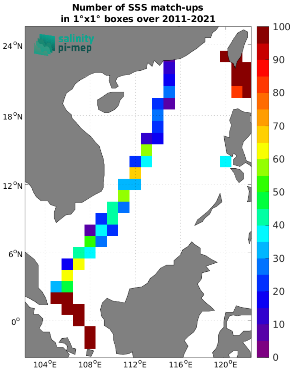
Figure 5: Number of SSS match-ups between TSG (LEGOS-DM) SSS and the SMAP SSS L4 OI v3 - Monthly (ESR) SSS product for the South China Sea Pi-MEP region over 1^\circ \times 1^\circ boxes and for the full satellite product period.
