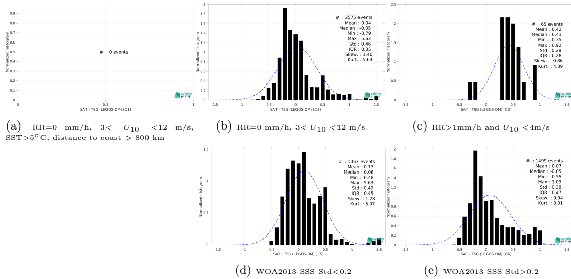
Figure 15: Normalized histogram of \Delta SSS (SMAP SSS L4 OI v3 - Monthly (ESR) - TSG (LEGOS-DM)) for 5 different subdatasets corresponding to: RR=0 mm/h, 3 < U_{10} < 12 m/s, SST > 5°C, distance to coast > 800 km (a), RR=0 mm/h, 3 < U_{10} < 12 m/s (b), RR > 1mm/h and U_{10} < 4 m/s (c), WOA2013 SSS Std < 0.2 (d), WOA2013 SSS Std > 0.2 (e).
