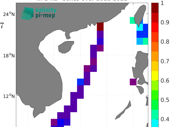
Temporal STD of (Sat - TSG (LEGOS-DM)) in 1°x1° boxes over 2011-2021
