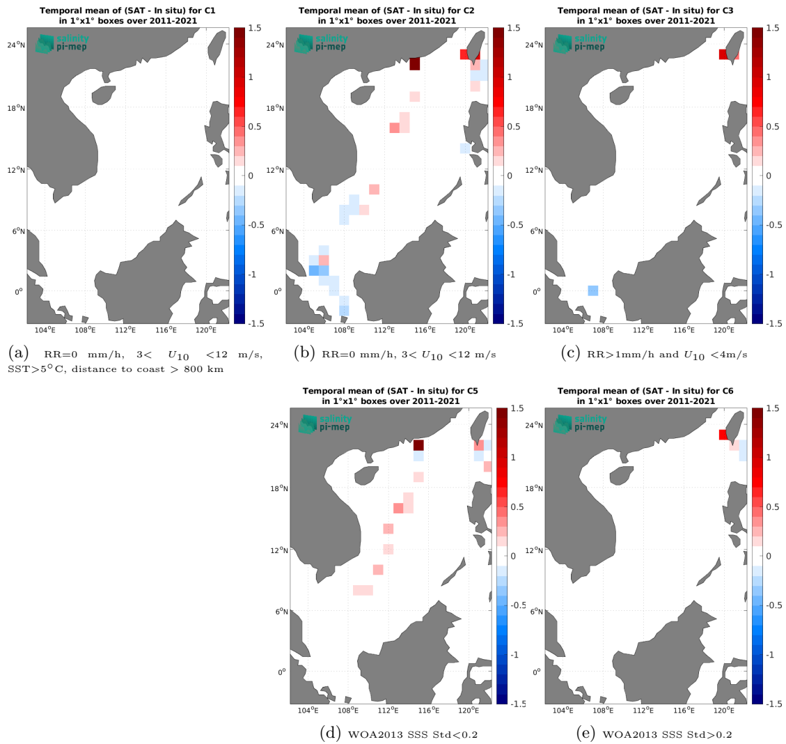
Figure 14: Temporal mean gridded over spatial boxes of size 1^\circ \times 1^\circ of \Delta\text{SSS} (SMAP SSS L4 OI v3 - Monthly (ESR) - TSG (LEGOS-DM)) for 5 different subdatasets corresponding to: RR=0 mm/h, 3 < U_{10} < 12 m/s, SST > 5^\circ\text{C} , distance to coast > 800 km (a), RR=0 mm/h, 3 < U_{10} < 12 m/s (b), RR > 1 mm/h and U_{10} < 4 m/s (c), WOA2013 SSS Std < 0.2 (d), WOA2013 SSS Std > 0.2 (e).
