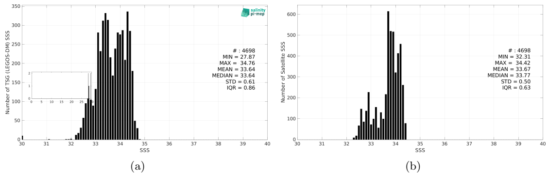
Figure 3: Histograms of SSS from TSG (LEGOS-DM) (a) and SMAP SSS L4 OI v3 - Monthly (ESR) (b) considering all match-up pairs per bins of 0.1 over the South China Sea Pi-MEP region and for the full satellite product period.
