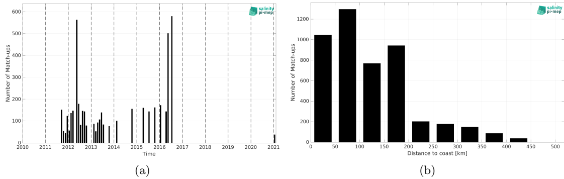
Figure 2: Number of match-ups between TSG (LEGOS-DM) and SMAP SSS L4 OI v3 - Monthly (ESR) SSS as a function of time (a) and as function of the distance to coast (b) over the South China Sea Pi-MEP region and for the full satellite product period.
