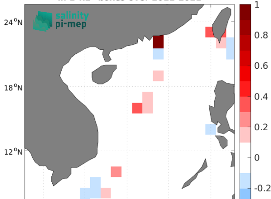
Temporal mean of (Sat - TSG (LEGOS-DM)) in 1°x1° boxes over 2011-2021
