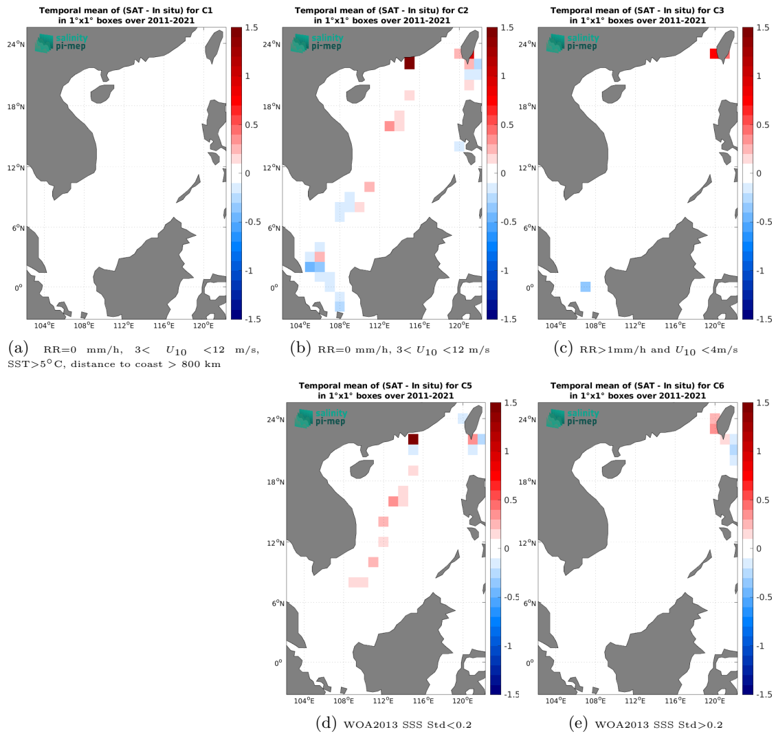
Figure 14: Temporal mean gridded over spatial boxes of size 1^{\circ}\times 1^{\circ} of \Delta SSS (SMAP SSS L4 OI v3 - Monthly (ESR) - TSG (LEGOS-DM)) for 5 different subdatasets corresponding to: RR=0 mm/h, 3 < U_{10} < 12 m/s, SST > 5^{\circ}C , distance to coast > 800 km (a), RR=0 mm/h, 3 < U_{10} < 12 m/s (b), RR > 1 mm/h and U_{10} < 4 m/s (c), WOA2013 SSS Std < 0.2 (d), WOA2013 SSS Std > 0.2 (e).
