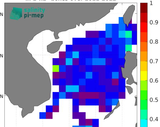
Temporal STD of (Sat - Argo) in 1°x1° boxes over 2011-2022
