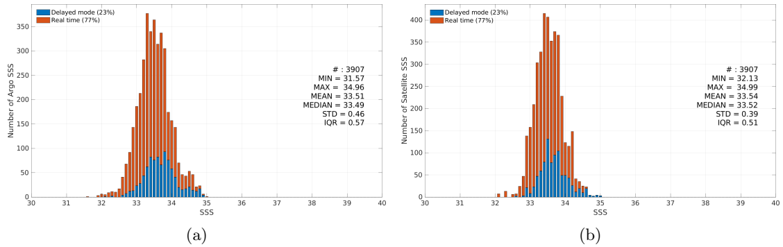
Figure 3: Histograms of SSS from Argo (a) and SMAP SSS L4 OI v3 - Monthly (ESR) (b) considering all match-up pairs per bins of 0.1 over the South China Sea Pi-MEP region and for the full satellite product period.
