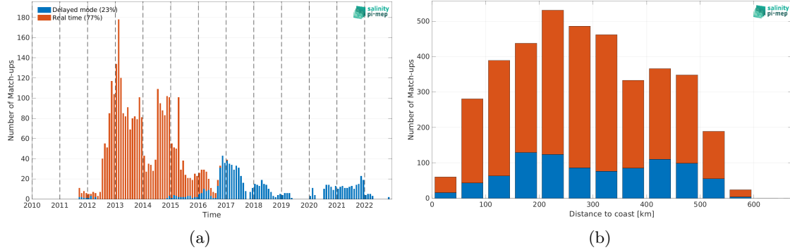
Figure 2: Number of match-ups between Argo and SMAP SSS L4 OI v3 - Monthly (ESR) SSS as a function of time (a) and as function of the distance to coast (b) over the South China Sea Pi-MEP region and for the full satellite product period.
