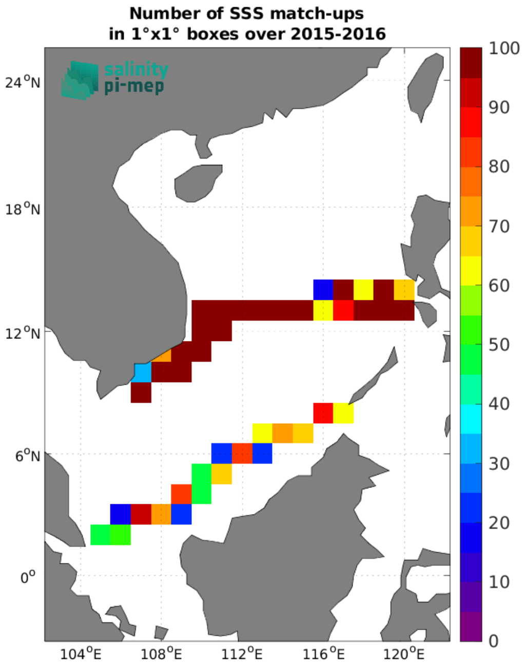
Figure 5: Number of SSS match-ups between TSG (SAMOS) SSS and the SMAP SSS L4 OI v3 - Daily (ESR) SSS product for the South China Sea Pi-MEP region over 1°x1° boxes and for the full satellite product period.
