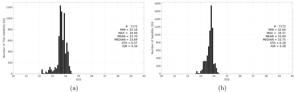
Figure 3: Histograms of SSS from TSG (SAMOS) (a) and SMAP SSS L4 OI v3 - Daily (ESR) (b) considering all match-up pairs per bins of 0.1 over the South China Sea Pi-MEP region and for the full satellite product period.
