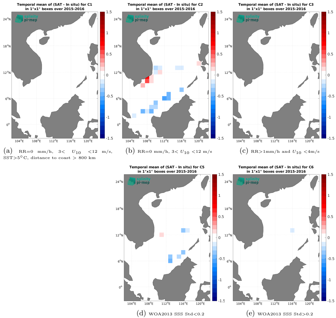
Figure 14: Temporal mean gridded over spatial boxes of size 1^\circ \times 1^\circ of \Delta\text{SSS} (SMAP SSS L4 OI v3 - Daily (ESR) - TSG (SAMOS)) for 5 different subdatasets corresponding to: RR=0 mm/h, 3 < U_{10} < 12 m/s, SST > 5^\circ\text{C} , distance to coast > 800 km (a), RR=0 mm/h, 3 < U_{10} < 12 m/s (b), RR > 1 mm/h and U_{10} < 4 m/s (c), WOA2013 SSS Std < 0.2 (d), WOA2013 SSS Std > 0.2 (e).
