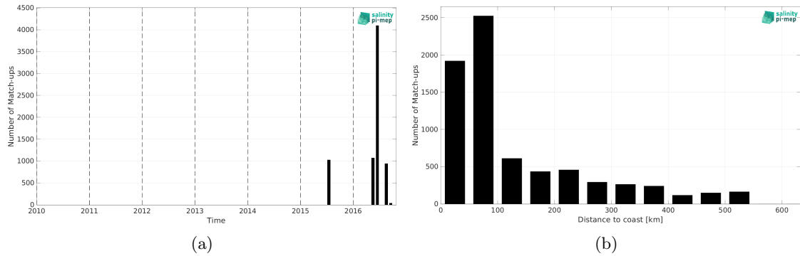
Figure 2: Number of match-ups between TSG (SAMOS) and SMAP SSS L4 OI v3 - Daily (ESR) SSS as a function of time (a) and as function of the distance to coast (b) over the South China Sea Pi-MEP region and for the full satellite product period.
