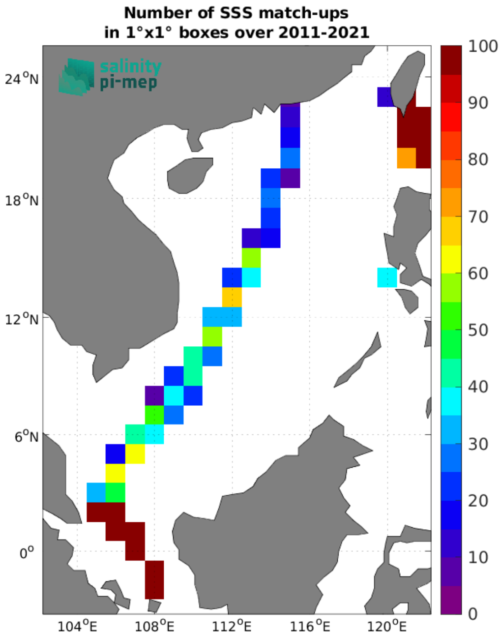
Figure 5: Number of SSS match-ups between TSG (LEGOS-DM) SSS and the SMAP SSS L4 OI v3 - Daily (ESR) SSS product for the South China Sea Pi-MEP region over 1^\circ \times 1^\circ boxes and for the full satellite product period.
