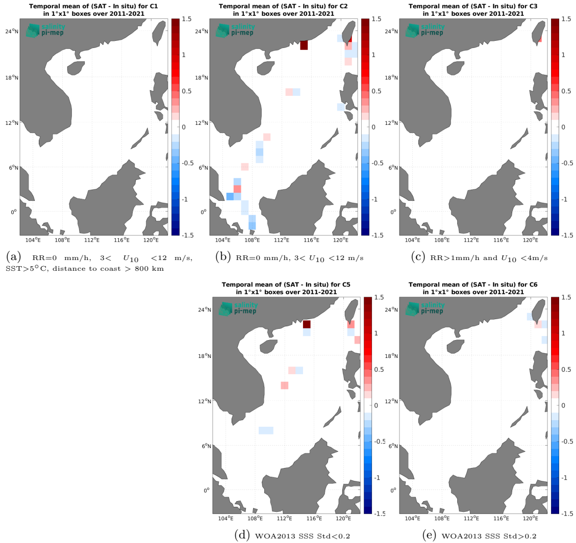
Figure 14: Temporal mean gridded over spatial boxes of size 1^\circ \times 1^\circ of \Delta\text{SSS} (SMAP SSS L4 OI v3 - Daily (ESR) - TSG (LEGOS-DM)) for 5 different subdatasets corresponding to: RR=0 mm/h, 3 < U_{10} < 12 m/s, SST > 5^\circ\text{C} , distance to coast > 800 km (a), RR=0 mm/h, 3 < U_{10} < 12 m/s (b), RR > 1 mm/h and U_{10} < 4 m/s (c), WOA2013 SSS Std < 0.2 (d), WOA2013 SSS Std > 0.2 (e).
