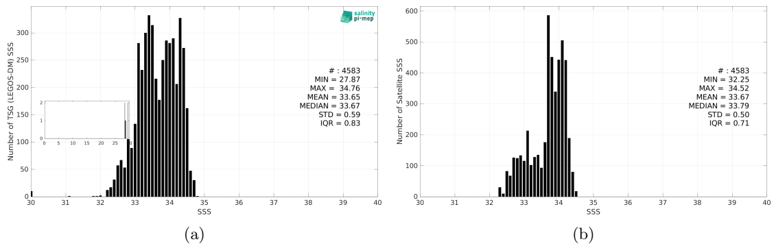
Figure 3: Histograms of SSS from TSG (LEGOS-DM) (a) and SMAP SSS L4 OI v3 - Daily (ESR) (b) considering all match-up pairs per bins of 0.1 over the South China Sea Pi-MEP region and for the full satellite product period.
