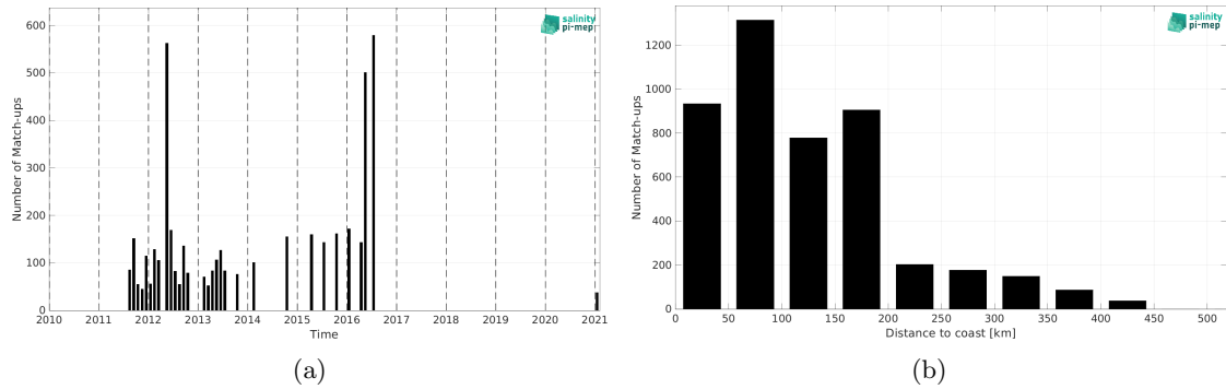
Figure 2: Number of match-ups between TSG (LEGOS-DM) and SMAP SSS L4 OI v3 - Daily (ESR) SSS as a function of time (a) and as function of the distance to coast (b) over the South China Sea Pi-MEP region and for the full satellite product period.
