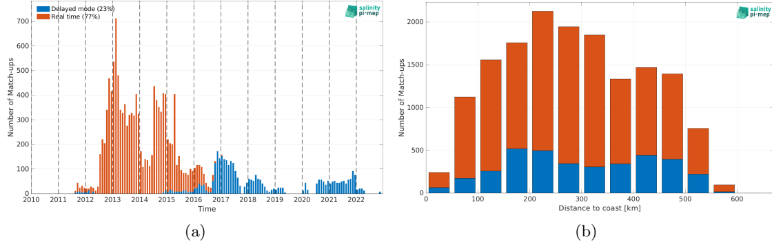
Figure 2: Number of match-ups between Argo and SMAP SSS L4 OI v3 - Daily (ESR) SSS as a function of time (a) and as function of the distance to coast (b) over the South China Sea Pi-MEP region and for the full satellite product period.
