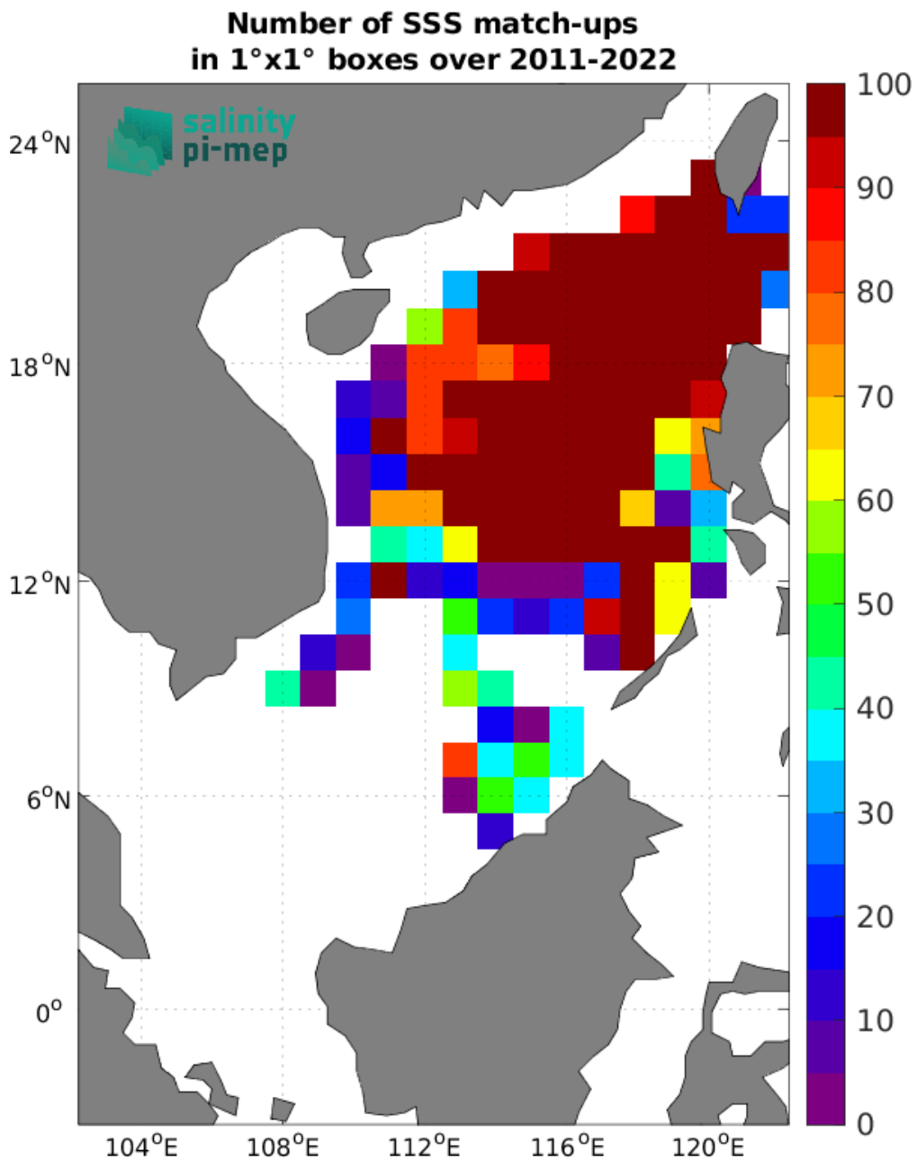
Figure 5: Number of SSS match-ups between Argo SSS and the SMAP SSS L4 OI v3 - Daily (ESR) SSS product for the South China Sea Pi-MEP region over 1^\circ \times 1^\circ boxes and for the full satellite product period.
