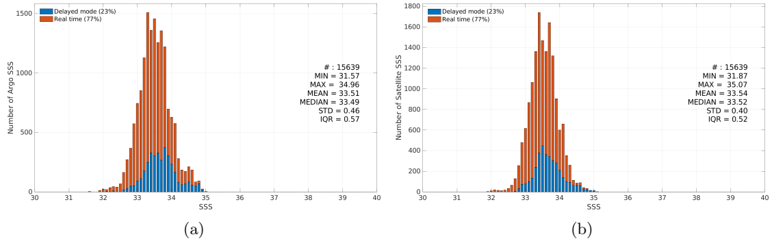
Figure 3: Histograms of SSS from Argo (a) and SMAP SSS L4 OI v3 - Daily (ESR) (b) considering all match-up pairs per bins of 0.1 over the South China Sea Pi-MEP region and for the full satellite product period.
