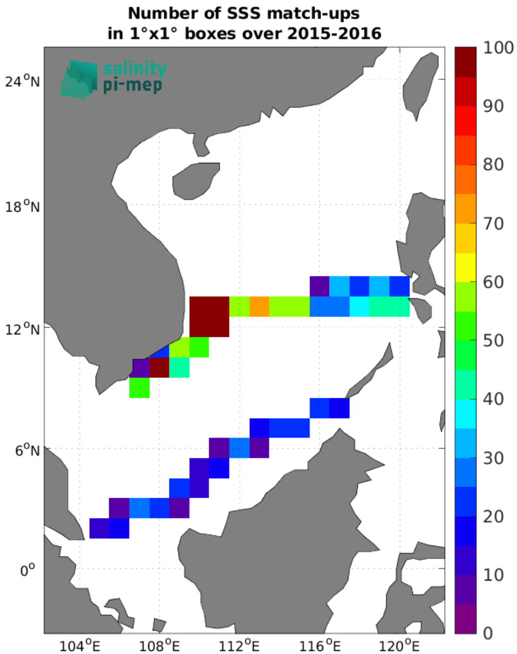
Figure 4: Number of SSS match-ups between TSG (SAMOS) SSS and the SMAP SSS L4 OI v2 - 7 Days (ESR) SSS product for the South China Sea Pi-MEP region over 1^{\circ} \times 1^{\circ} boxes and for the full satellite product period.
