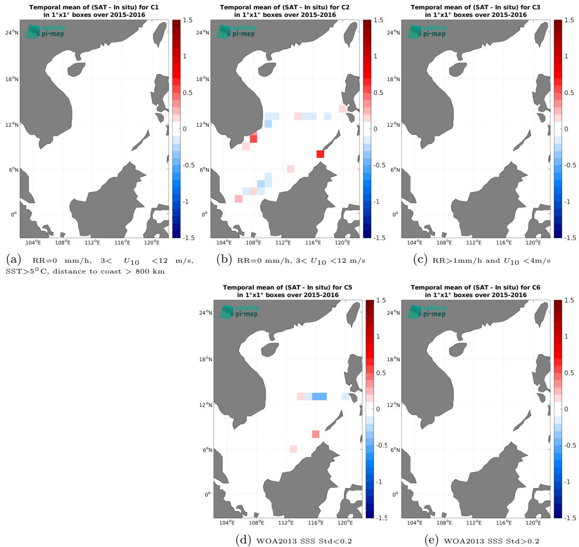
Figure 12: Temporal mean gridded over spatial boxes of size 1^\circ \times 1^\circ of \Delta\text{SSS} (SMAP SSS L4 OI v2 - 7 Days (ESR) - TSG (SAMOS)) for 5 different subdatasets corresponding to:RR=0 mm/h, 3 < U_{10} < 12 m/s, SST >5^\circ\text{C} , distance to coast > 800 km (a), RR=0 mm/h, 3 < U_{10} < 12 m/s (b), RR >1 mm/h and U_{10} < 4 m/s (c), WOA2013 SSS Std <0.2 (d), WOA2013 SSS Std >0.2 (e).
