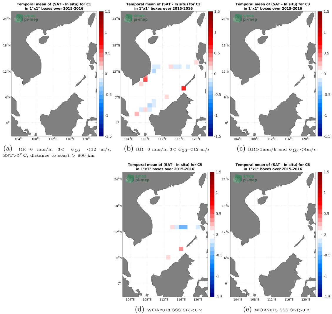
Figure 12: Temporal mean gridded over spatial boxes of size 1^\circ \times 1^\circ of \Delta SSS (SMAP SSS L4 OI v2 - 7 Days (ESR) - TSG (SAMOS)) for 5 different subdatasets corresponding to:RR=0 mm/h, 3 < U_{10} < 12 m/s, SST>5°C, distance to coast > 800 km (a), RR=0 mm/h, 3 < U_{10} < 12 m/s (b), RR>1mm/h and U_{10} < 4 m/s (c), WOA2013 SSS Std<0.2 (d), WOA2013 SSS Std>0.2 (e).
