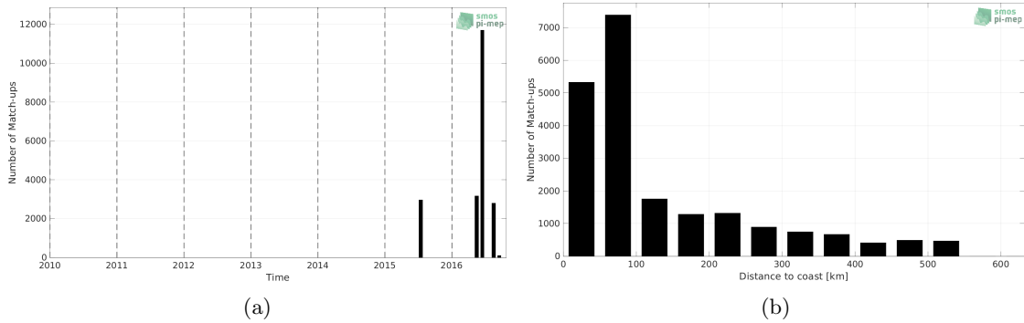
Figure 1: Number of match-ups between TSG (SAMOS) and SMAP SSS L4 OI v2 - 7 Days (ESR) SSS as a function of time (a) and as function of the distance to coast (b) over the South China Sea Pi-MEP region and for the full satellite product period.
