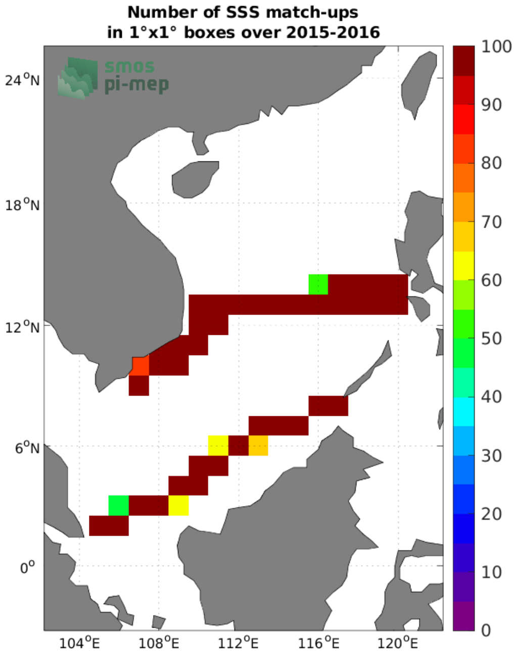
Figure 4: Number of SSS match-ups between TSG (SAMOS) SSS and the SMAP SSS L4 OI v2 - 7 Days (ESR) SSS product for the South China Sea Pi-MEP region over 1°x1° boxes and for the full satellite product period.
