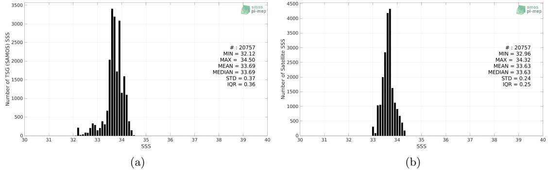
Figure 2: Histograms of SSS from TSG (SAMOS) (a) and SMAP SSS L4 OI v2 - 7 Days (ESR) (b) considering all match-up pairs per bins of 0.1 over the South China Sea Pi-MEP region and for the full satellite product period.
