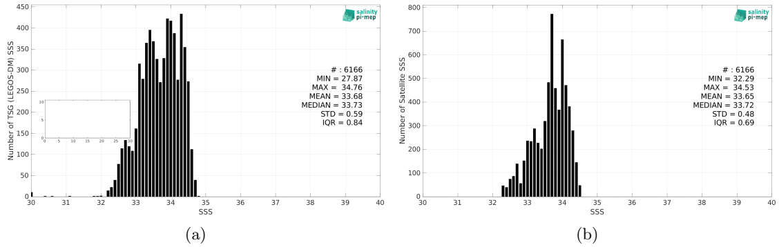
Figure 2: Histograms of SSS from TSG (LEGOS-DM) (a) and SMAP SSS L4 OI v2 - 7 Days (ESR) (b) considering all match-up pairs per bins of 0.1 over the South China Sea Pi-MEP region and for the full satellite product period.
