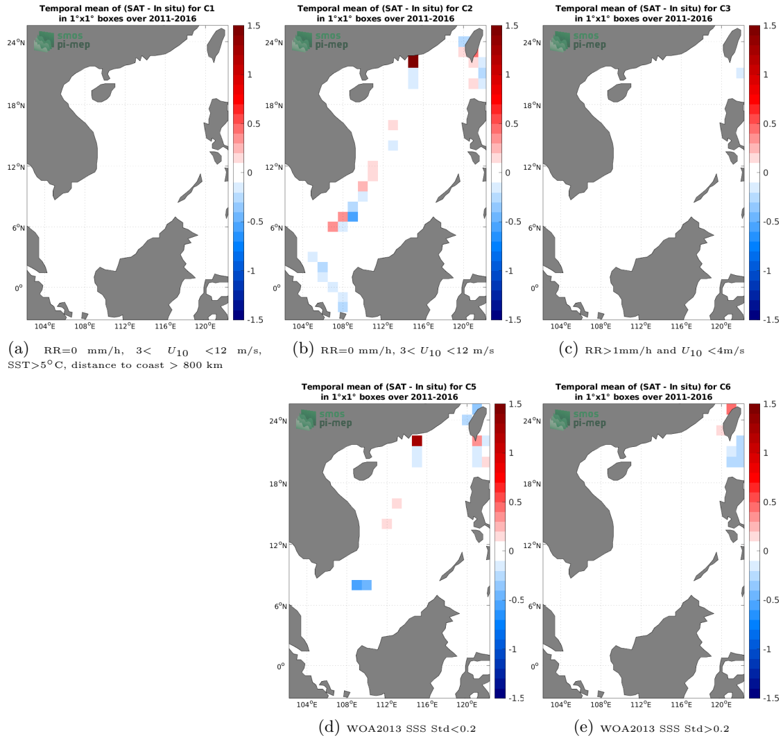
Figure 12: Temporal mean gridded over spatial boxes of size 1^\circ \times 1^\circ of \Delta SSS (SMAP SSS L4 OI v2 - 7 Days (ESR) - TSG (LEGOS-DM)) for 5 different subdatasets corresponding to: RR=0 mm/h, 3 < U_{10} < 12 m/s, SST>5°C, distance to coast > 800 km (a), RR=0 mm/h, 3 < U_{10} < 12 m/s (b), RR>1mm/h and U_{10} < 4 m/s (c), WOA2013 SSS Std<0.2 (d), WOA2013 SSS Std>0.2 (e).
