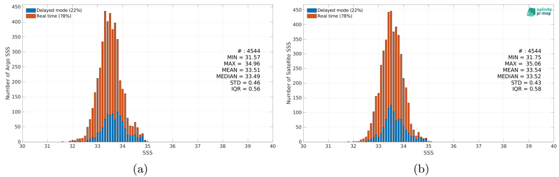
Figure 2: Histograms of SSS from Argo (a) and SMAP SSS L4 OI v2 - 7 Days (ESR) (b) considering all match-up pairs per bins of 0.1 over the South China Sea Pi-MEP region and for the full satellite product period.
