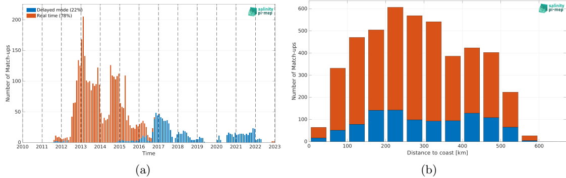
Figure 1: Number of match-ups between Argo and SMAP SSS L4 OI v2 - 7 Days (ESR) SSS as a function of time (a) and as function of the distance to coast (b) over the South China Sea Pi-MEP region and for the full satellite product period.
