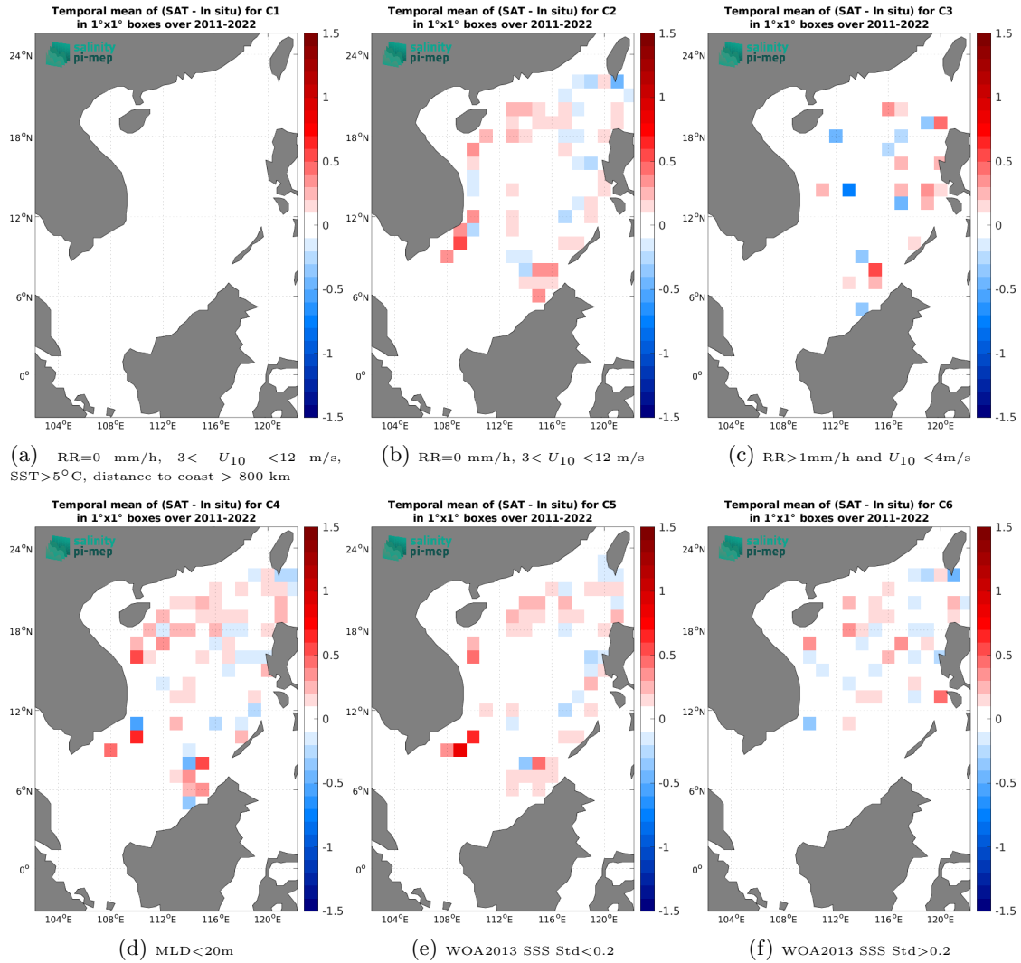
Figure 12: Temporal mean gridded over spatial boxes of size 1^\circ \times 1^\circ of \Delta SSS (SMAP SSS L4 OI v2 - 7 Days (ESR) - Argo) for 6 different subdatasets corresponding to:RR=0 mm/h, 3 < U_{10} < 12 m/s, SST>5°C, distance to coast > 800 km (a), RR=0 mm/h, 3 < U_{10} < 12 m/s (b), RR>1mm/h and U_{10} < 4 m/s (c),MLD<20m (d),WOA2013 SSS Std<0.2 (e),WOA2013 SSS Std>0.2 (f).
