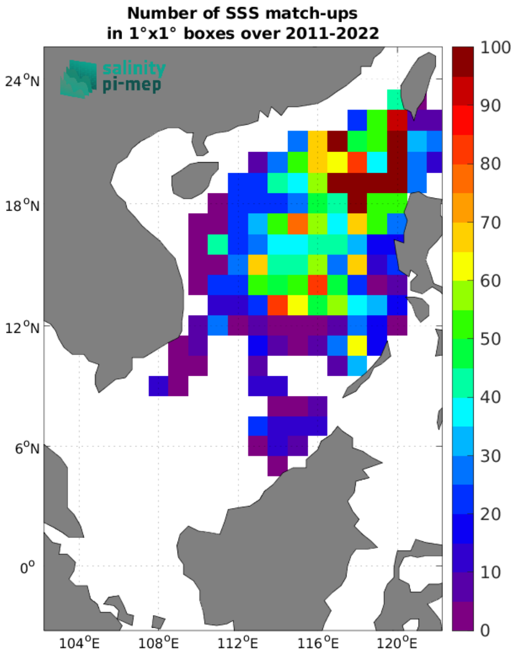
Figure 4: Number of SSS match-ups between Argo SSS and the SMAP SSS L4 OI v2 - 7 Days (ESR) SSS product for the South China Sea Pi-MEP region over 1^\circ \times 1^\circ boxes and for the full satellite product period.
