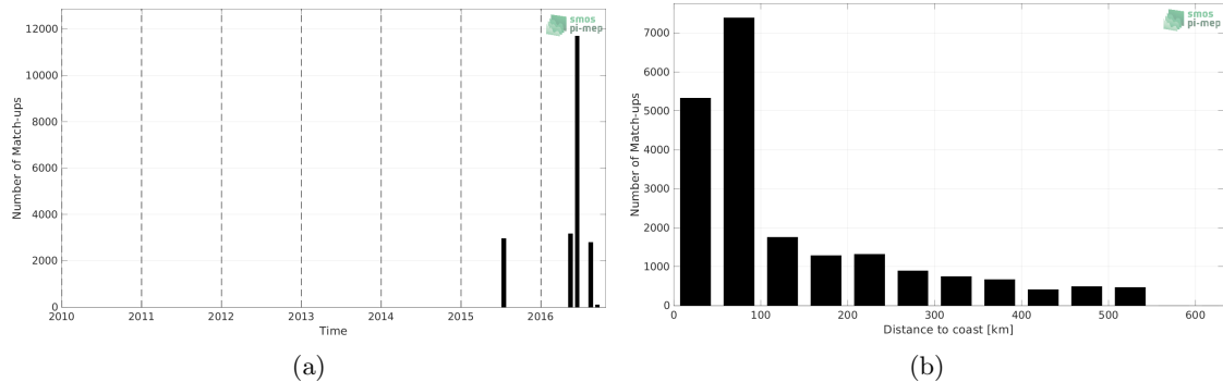
Figure 1: Number of match-ups between TSG (SAMOS) and SMAP SSS L4 OI v2 - Monthly (IPRC) SSS as a function of time (a) and as function of the distance to coast (b) over the South China Sea Pi-MEP region and for the full satellite product period.
