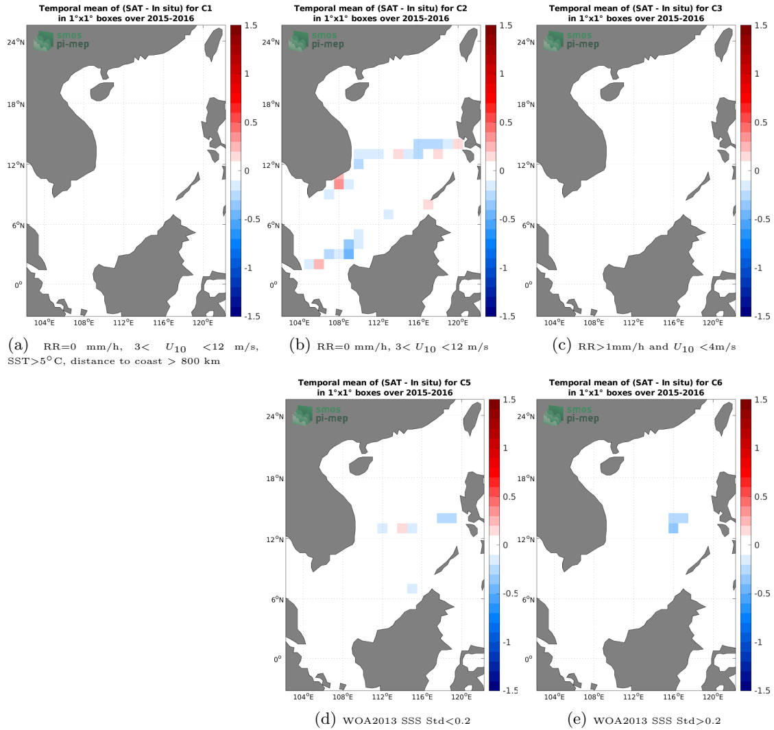
Figure 12: Temporal mean gridded over spatial boxes of size 1^\circ \times 1^\circ of \Delta SSS (SMAP SSS L4 OI v2 - Monthly (IPRC) - TSG (SAMOS)) for 5 different subdatasets corresponding to: RR=0 mm/h, 3 < U_{10} < 12 m/s, SST>5°C, distance to coast > 800 km (a), RR=0 mm/h, 3 < U_{10} < 12 m/s (b), RR>1mm/h and U_{10} < 4 m/s (c), WOA2013 SSS Std<0.2 (d), WOA2013 SSS Std>0.2 (e).
