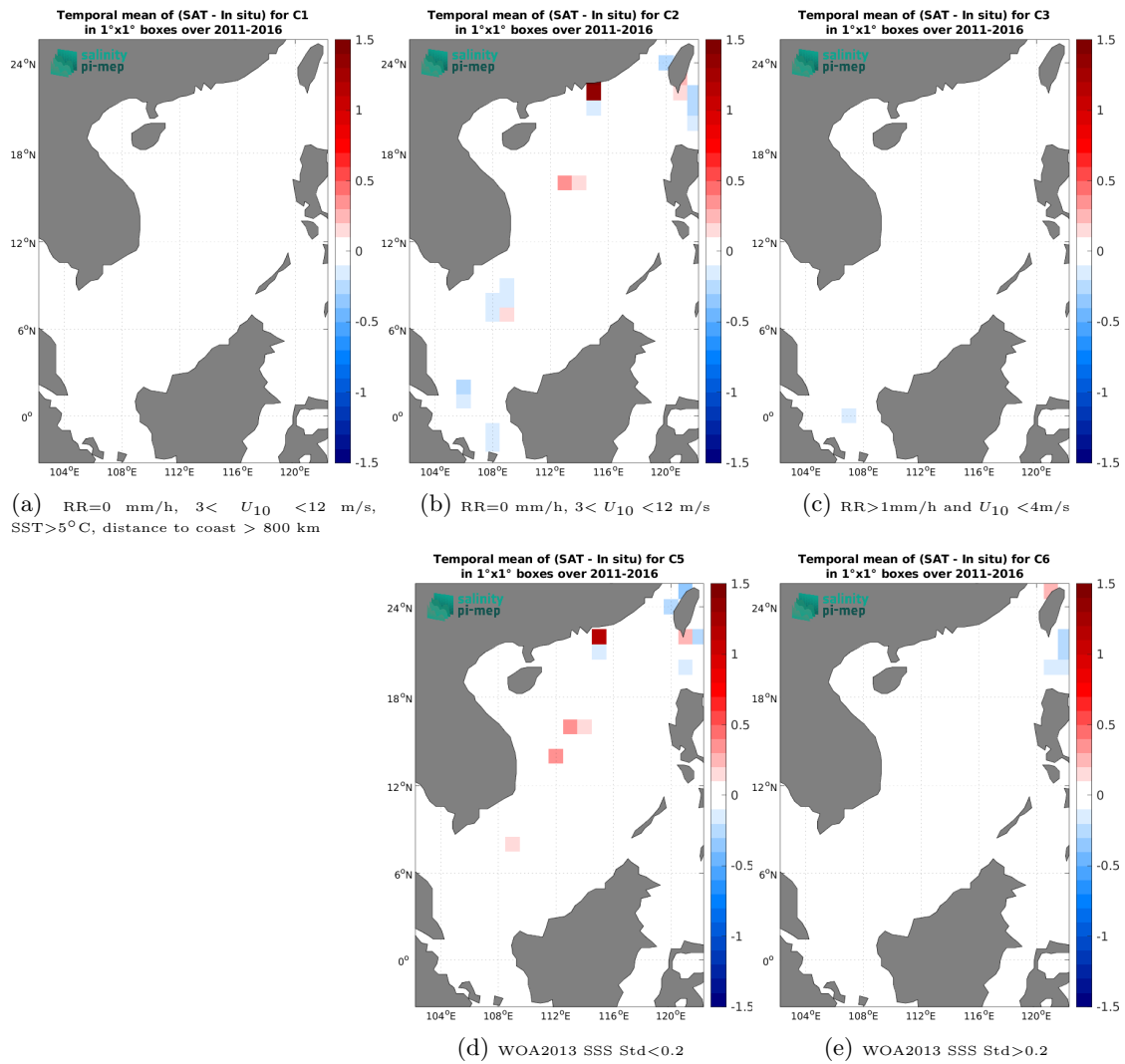
Figure 12: Temporal mean gridded over spatial boxes of size 1^\circ \times 1^\circ of \Delta SSS (SMAP SSS L4 OI v2 - Monthly (IPRC) - TSG (LEGOS-DM)) for 5 different subdatasets corresponding to:RR=0 mm/h, 3 < U_{10} < 12 m/s, SST>5°C, distance to coast > 800 km (a), RR=0 mm/h, 3 < U_{10} < 12 m/s (b), RR>1mm/h and U_{10} < 4 m/s (c), WOA2013 SSS Std<0.2 (d), WOA2013 SSS Std>0.2 (e).
