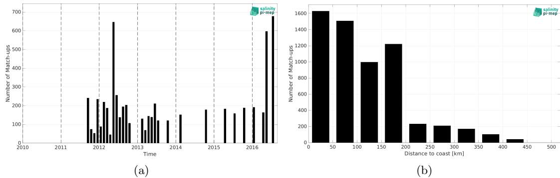
Figure 1: Number of match-ups between TSG (LEGOS-DM) and SMAP SSS L4 OI v2 - Monthly (IPRC) SSS as a function of time (a) and as function of the distance to coast (b) over the South China Sea Pi-MEP region and for the full satellite product period.
