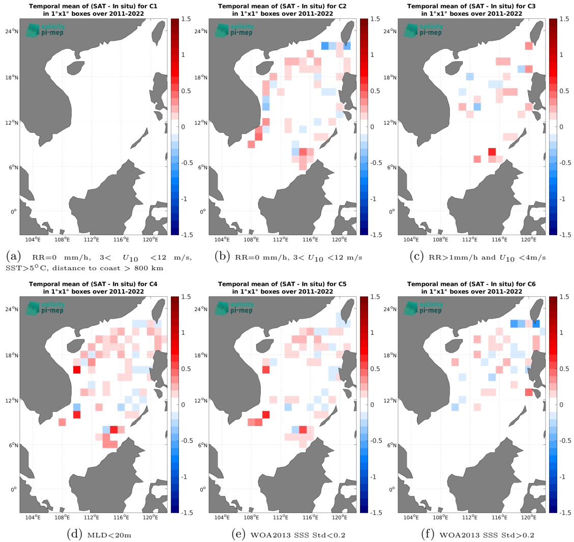
Figure 12: Temporal mean gridded over spatial boxes of size 1^\circ \times 1^\circ of \Delta SSS (SMAP SSS L4 OI v2 - Monthly (IPRC) - Argo) for 6 different subdatasets corresponding to:RR=0 mm/h, 3 < U_{10} < 12 m/s, SST>5°C, distance to coast > 800 km (a), RR=0 mm/h, 3 < U_{10} < 12 m/s (b), RR>1mm/h and U_{10} < 4 m/s (c),MLD<20m (d),WOA2013 SSS Std<0.2 (e),WOA2013 SSS Std>0.2 (f).
