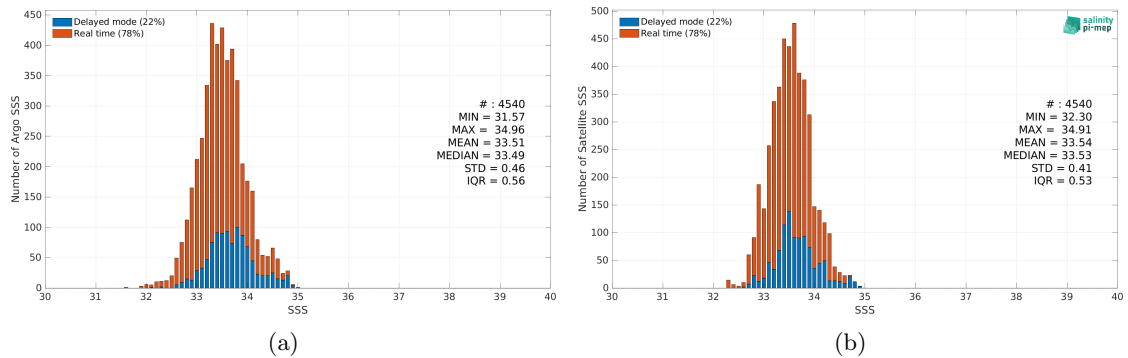
Figure 2: Histograms of SSS from Argo (a) and SMAP SSS L4 OI v2 - Monthly (IPRC) (b) considering all match-up pairs per bins of 0.1 over the South China Sea Pi-MEP region and for the full satellite product period.
