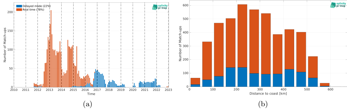
Figure 1: Number of match-ups between Argo and SMAP SSS L4 OI v2 - Monthly (IPRC) SSS as a function of time (a) and as function of the distance to coast (b) over the South China Sea Pi-MEP region and for the full satellite product period.
