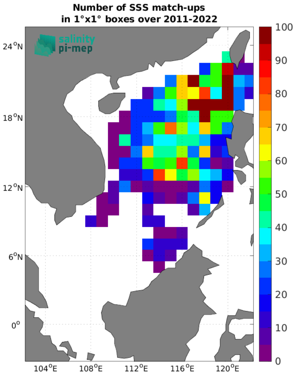
Figure 4: Number of SSS match-ups between Argo SSS and the SMAP SSS L4 OI v2 - Monthly (IPRC) SSS product for the South China Sea Pi-MEP region over 1^\circ \times 1^\circ boxes and for the full satellite product period.
